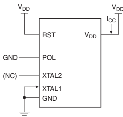
Figure 25-20. Connection Diagram for I CC Power-down Measurement. All Other Pins are Disconnected, V_{DD} = 2\text{V to } 5.5\text{V}
