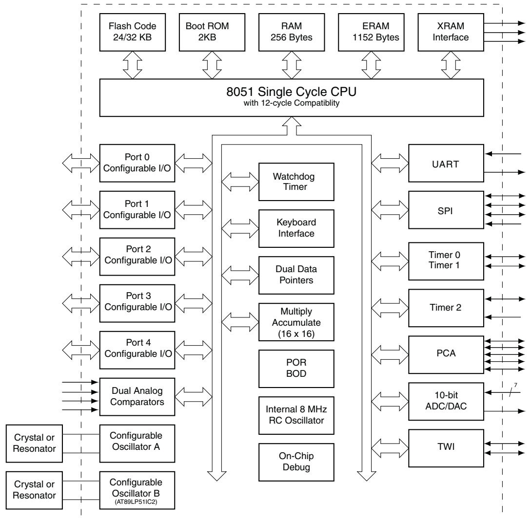
Figure 2-1. Atmel AT89LP51RB2/RC2/IC2 Block Diagram
