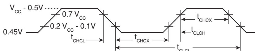
Figure 25-19. Clock Signal Waveform for I CC in Active and Idle Modes, t_{CLCH} = t_{CHCL} = 5 \text{ ns}
