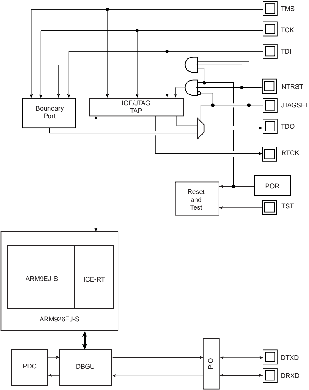
Figure 10-1. Debug and Test Block Diagram
