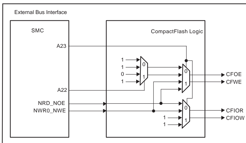
Figure 18-4. CompactFlash Read/Write Control Signals
