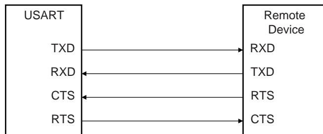
Figure 30-17. Connection with a Remote Device for Hardware Handshaking
