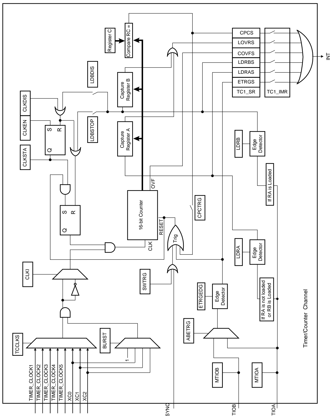
Figure 32-5. Capture Mode
