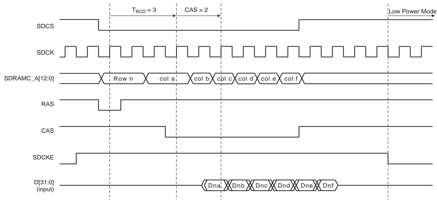
Figure 20-7. Low-power Mode Behavior
