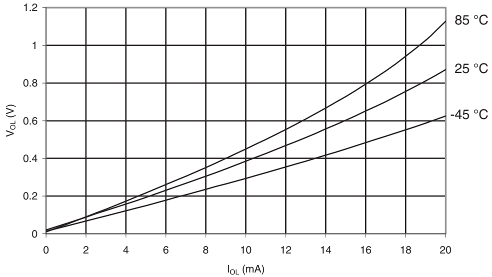
Figure 30-580. ATmega6450P: I/O Pin Output Voltage vs. Sink Current, Port B ( V_{CC} = 2.7V )
