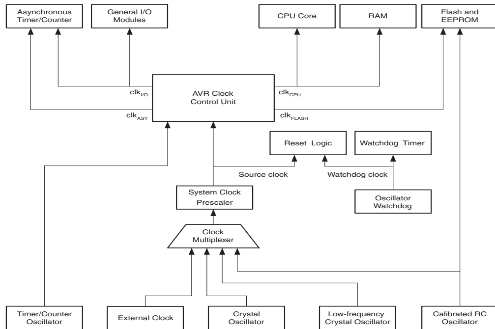
Figure 9-1. Clock distribution.
