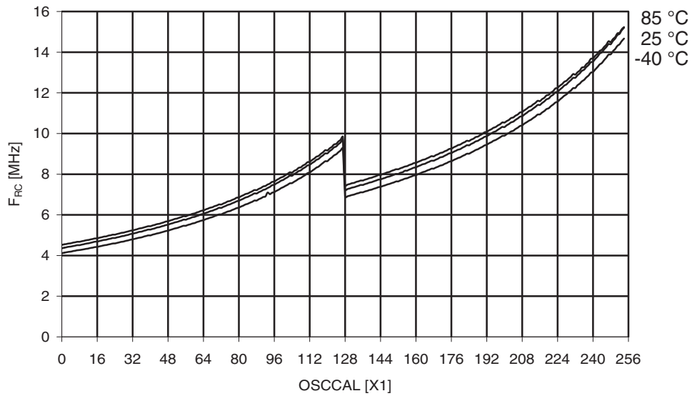
Figure 30-353. ATmega3250PA: Calibrated 8MHz RC Oscillator Frequency vs. Oscscal Value
