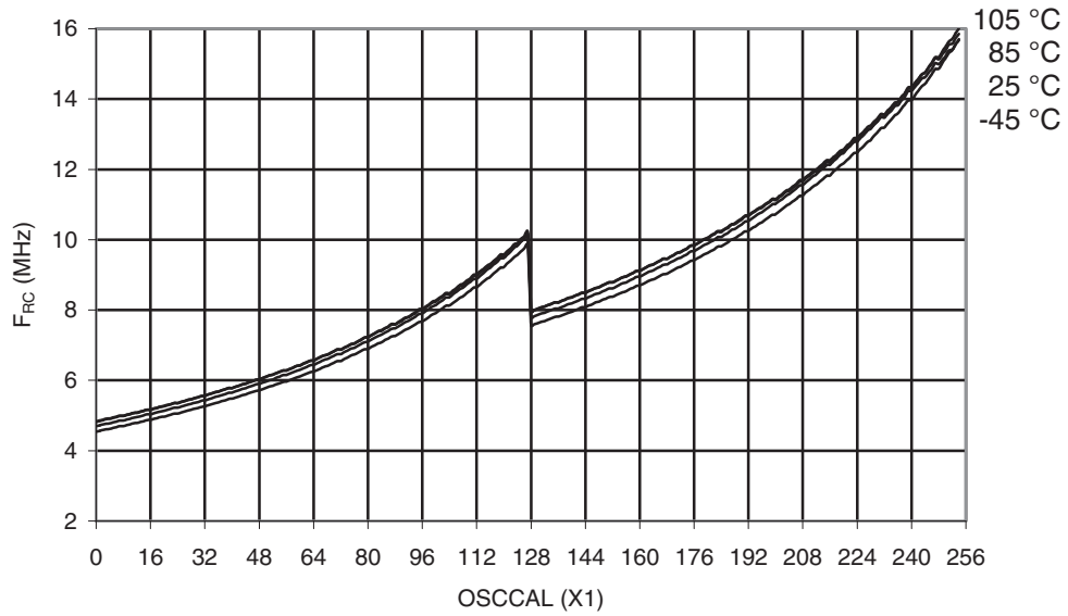
Figure 31-48. ATmega165PA: Calibrated 8MHz RC Oscillator Frequency vs. Oscscal Value
