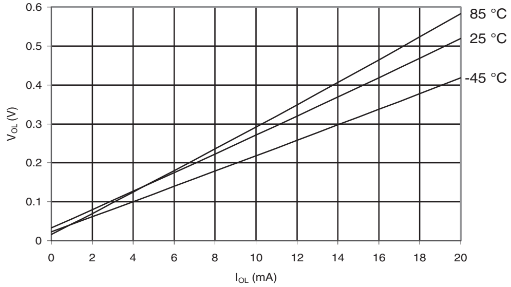
Figure 30-576. ATmega6450A: I/O Pin Output Voltage vs. Sink Current, Ports A, C, D, E, F, G, H ( V_{CC} = 5V )
