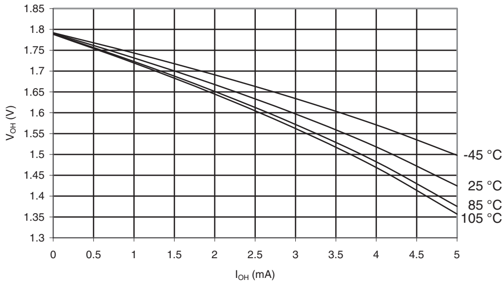
Figure 31-27. ATmega165PA: I/O Pin Output Voltage vs. Source Current, Port B ( V_{CC} = 1.8V )
