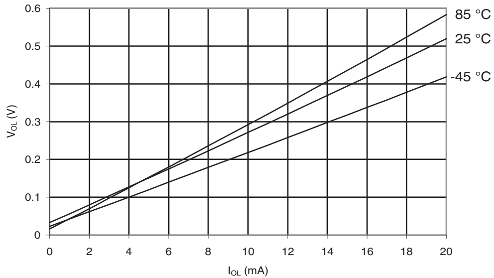
Figure 30-396. ATmega645A: I/O Pin Output Voltage vs. Sink Current, Port B ( V_{CC} = 5V )
