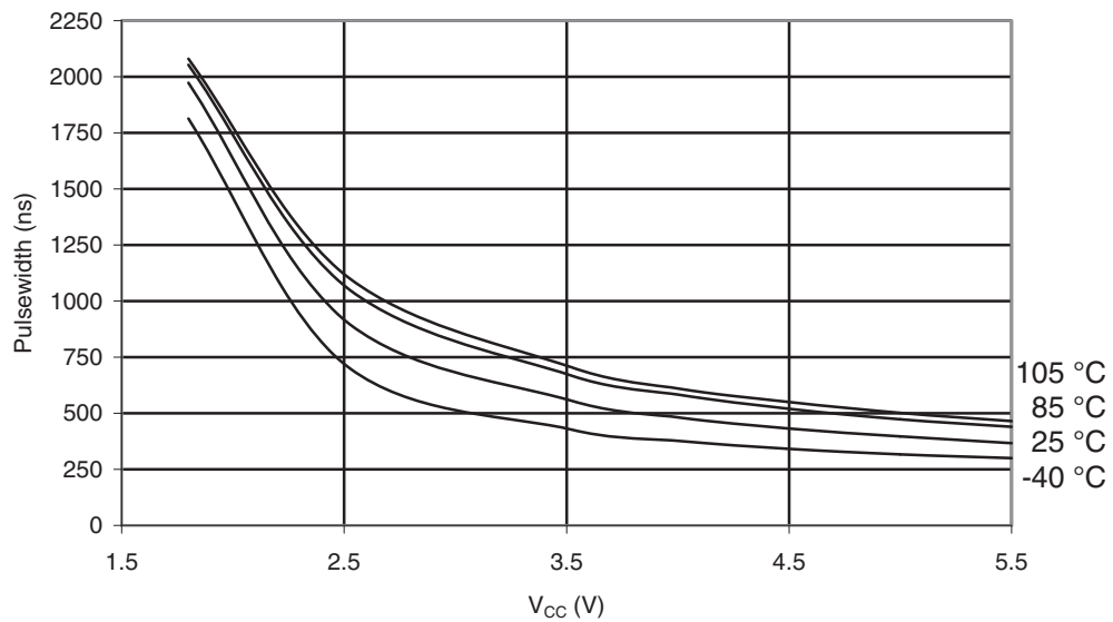
Figure 31-239. ATmega3250P: Minimum Reset Pulse Width vs. V_{CC}
