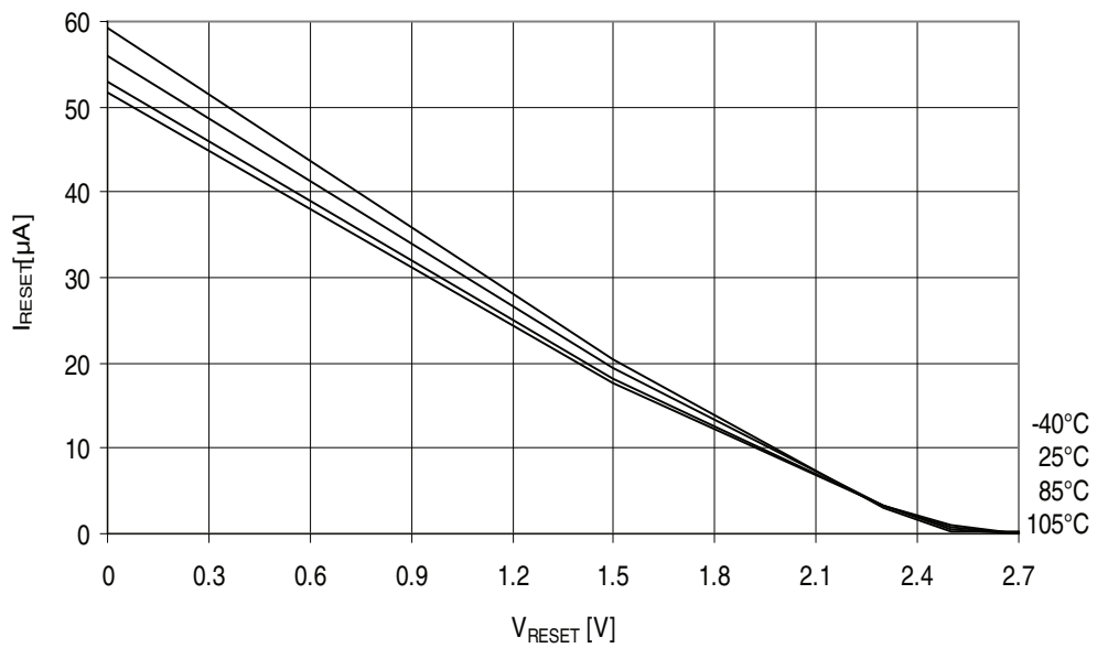
Figure 31-143. ATmega325PA: Reset Pull-up Resistor Current vs. Reset Pin Voltage ( V_{CC} = 2.7V )
