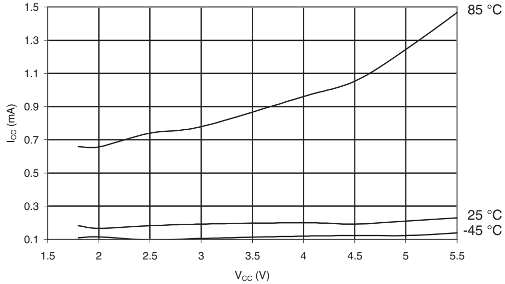
Figure 30-499. ATmega6450A: Power-down Supply Current vs. V_{CC} (32kHz Watch XTAL)
