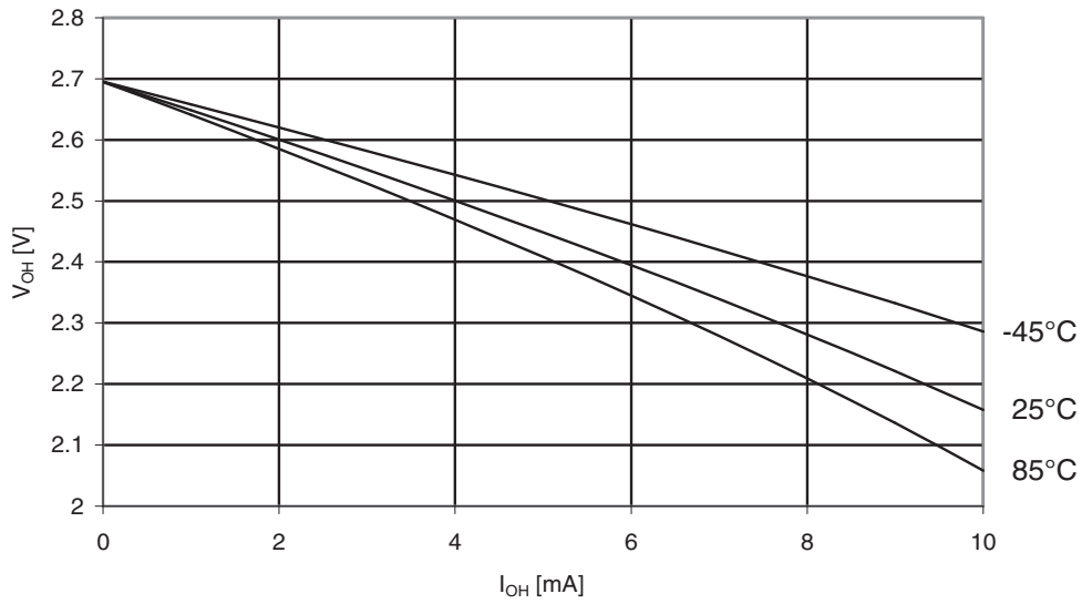
Figure 30-23. Atmel ATmega165A: I/O pin output voltage vs. source current, Ports A, C, D, E, F, G ( V_{CC} = 2.7V ).
