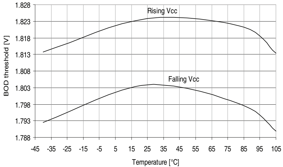
Figure 31-345. ATmega3250PA: BOD Thresholds vs. Temperature (BOD Level is 1.8V)
