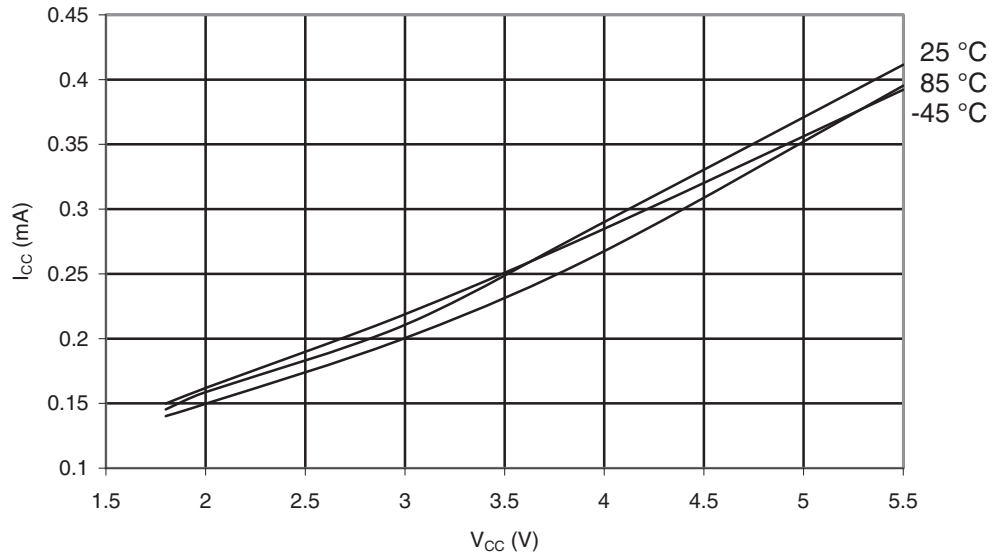
Figure 30-370. ATmega645A: Idle Supply Current vs. Low Frequency (0.1 - 1.0MHz)
