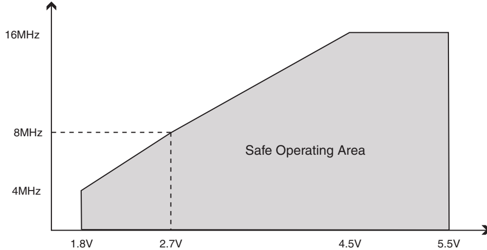
Figure 28-1. Maximum frequency vs. V_{CC} , Atmel ATmega165A/165PA/ATmega645A/ATmega645P.
