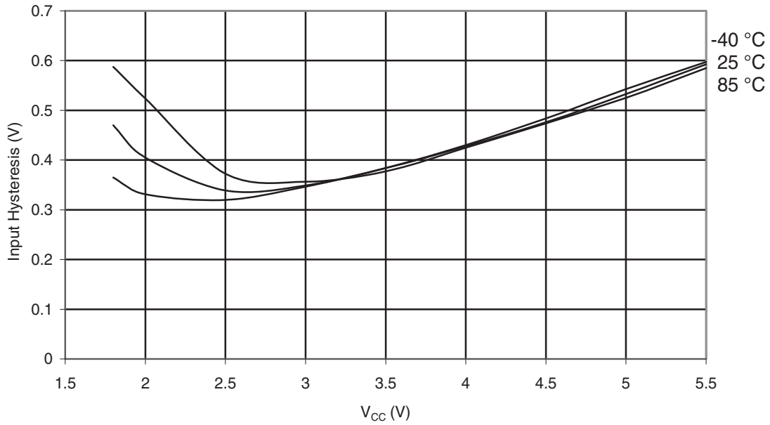
Figure 31-311. ATmega328: I/O Pin Input Hysteresis vs. V_{CC}
