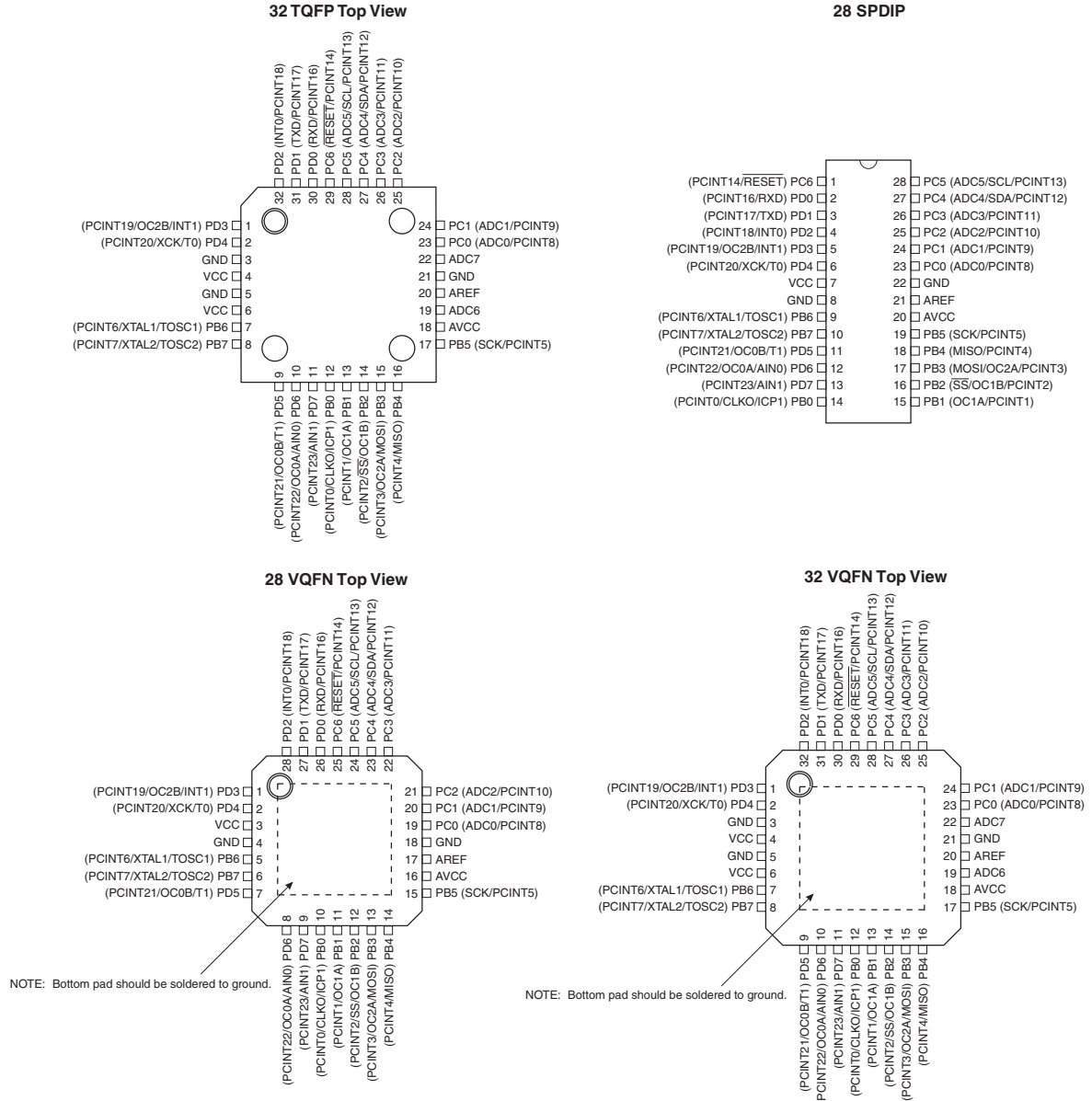
Figure 1-1. Pinout ATmega48A/PA/88A/PA/168A/PA/328/P
