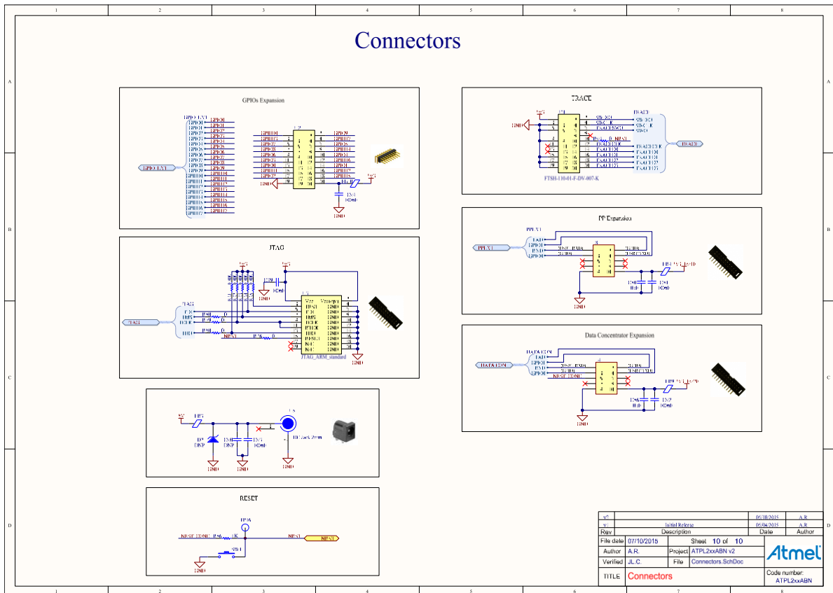
Figure A-10. ATPL250ABN Connectors.
