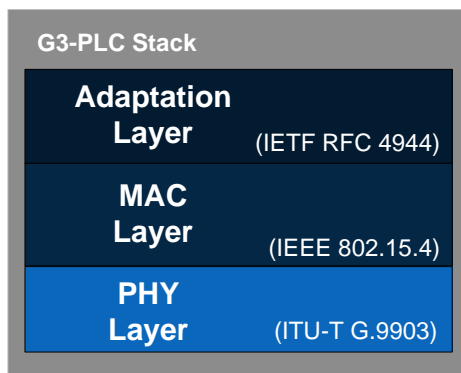
Figure 7-51. G3- PLC stack.
