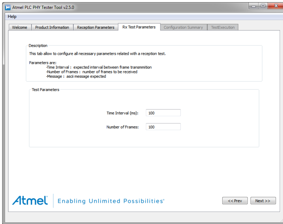
Figure 7-22. RX test parameters.
