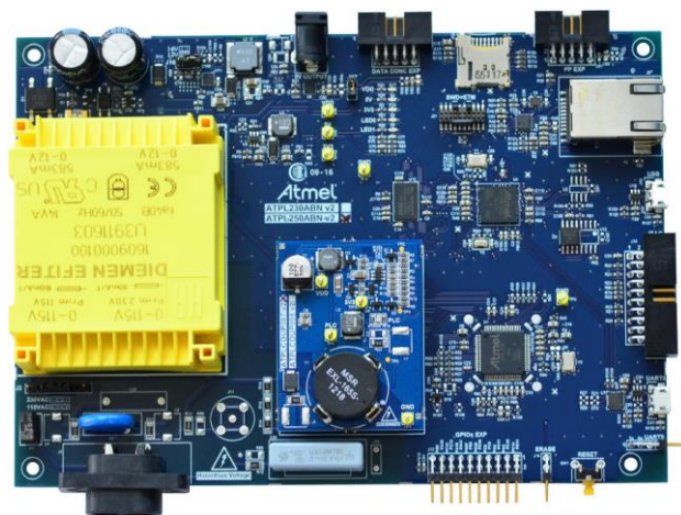
Figure 2-2. ATPL250ABN PAN Coordinator board and with ATPLCOUP007.
