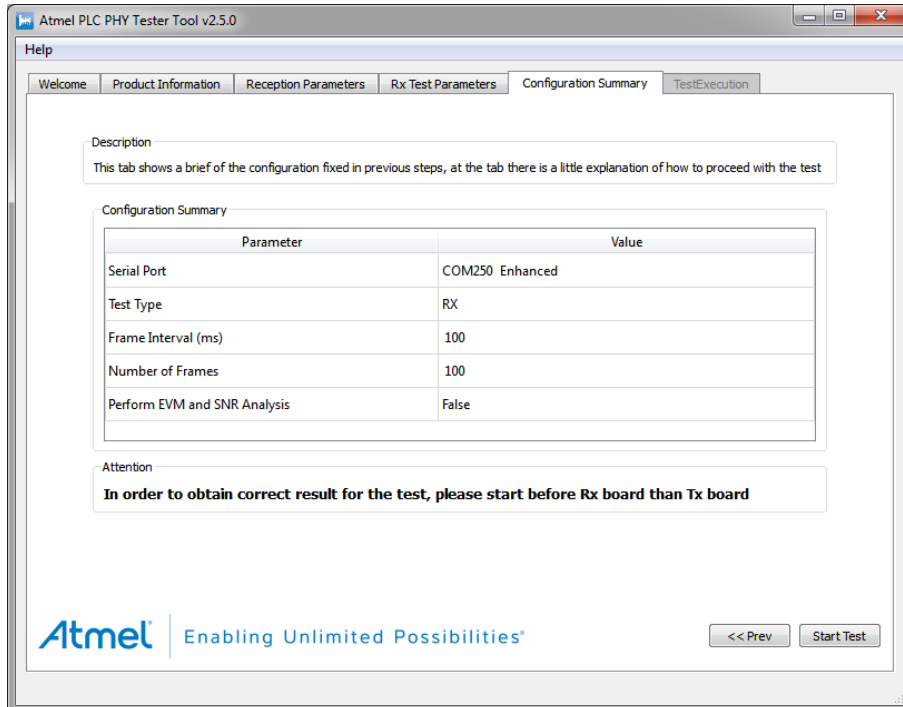
Figure 7-23. Configuration Summary tab.
