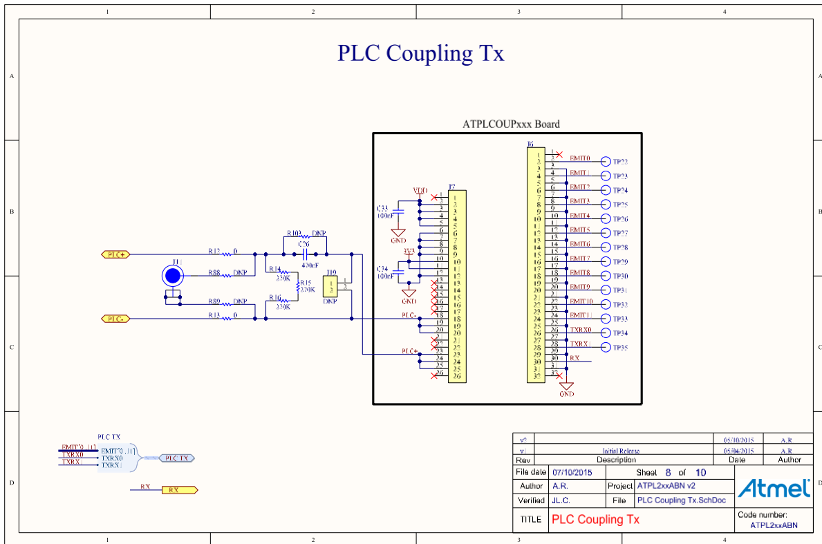
Figure A-8. ATPL250ABN PLC Coupling transmission scheme.
