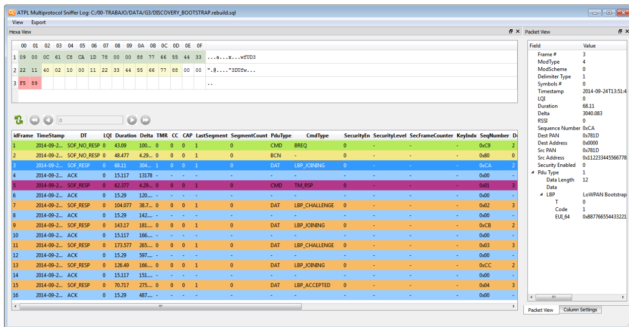
Figure 7-48. ATPL Multiprotocol Sniffer tool main window.
