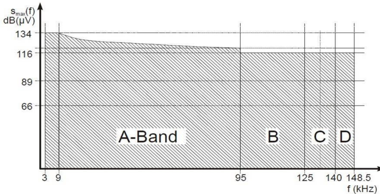
Figure 4-1. CENELEC bands.
