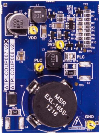
Figure 2-4. ATPLCOUP002 Coupling board.
