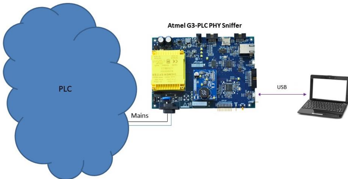
Figure 7-38. ATPL250ABN board connection scheme.
