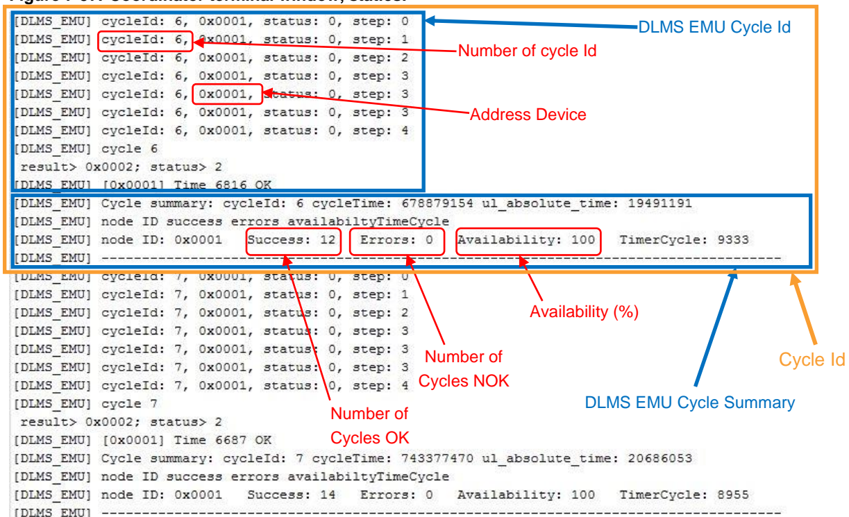
Figure 7-57. Coordinator terminal window, statics.
