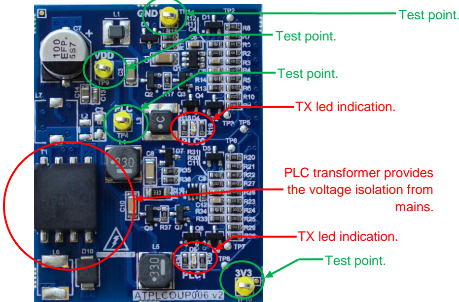
Figure 6-2. ATPLCOUP006v2 PLC coupling board.
