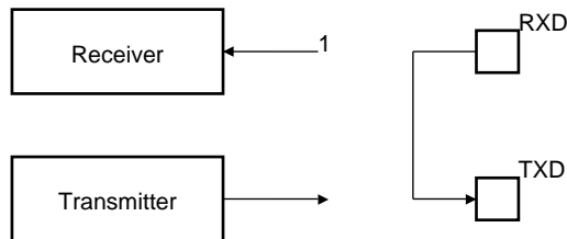
Figure 24-58. Remote Loopback Mode Configuration
