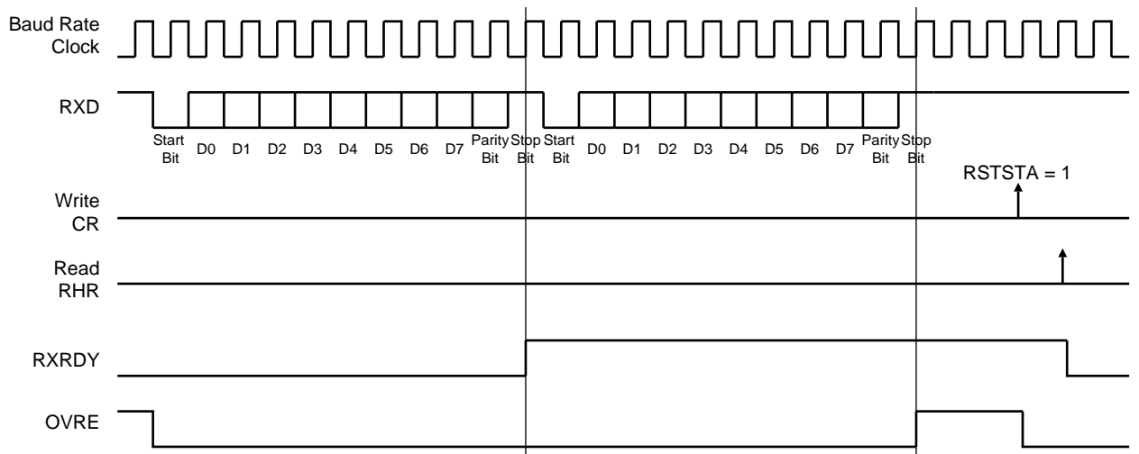
Figure 24-8. Receiver Status
