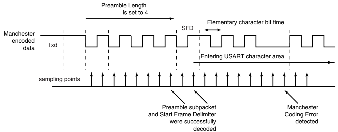
Figure 24-51. Manchester Error
