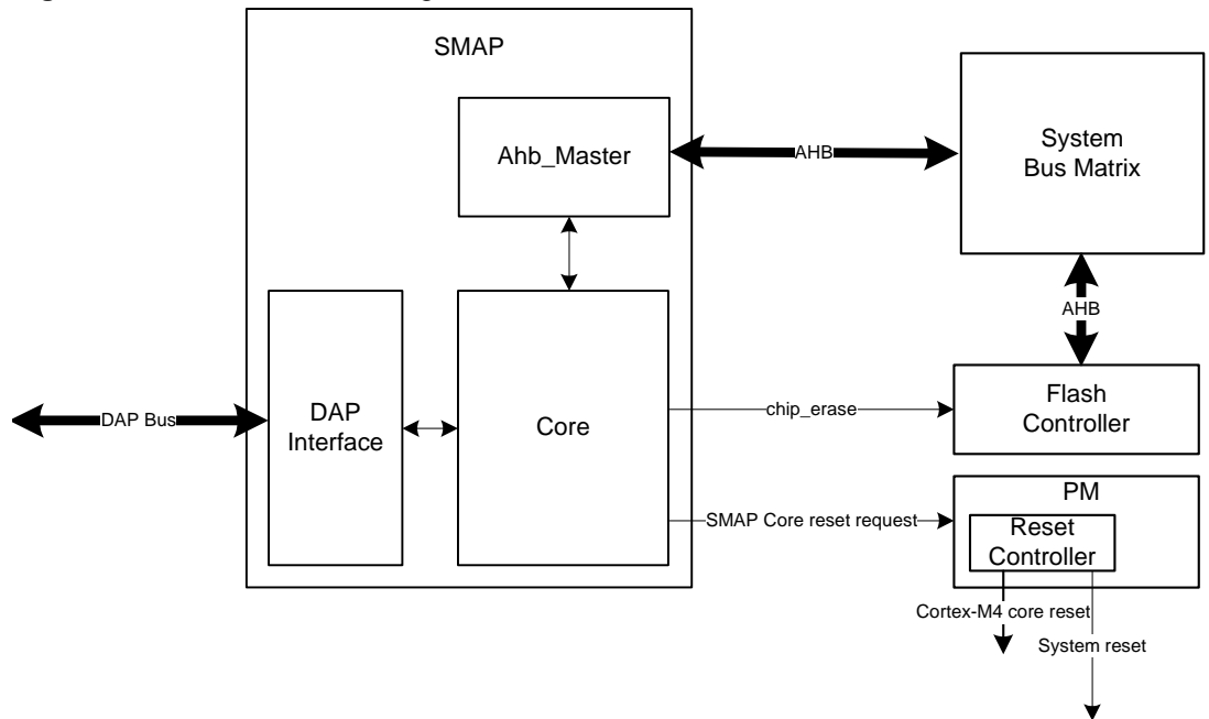
Figure 8-7. SMAP Block Diagram
