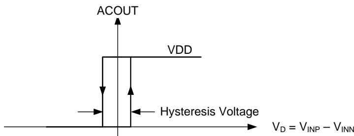
Figure 37-3. Hysteresis Voltage
