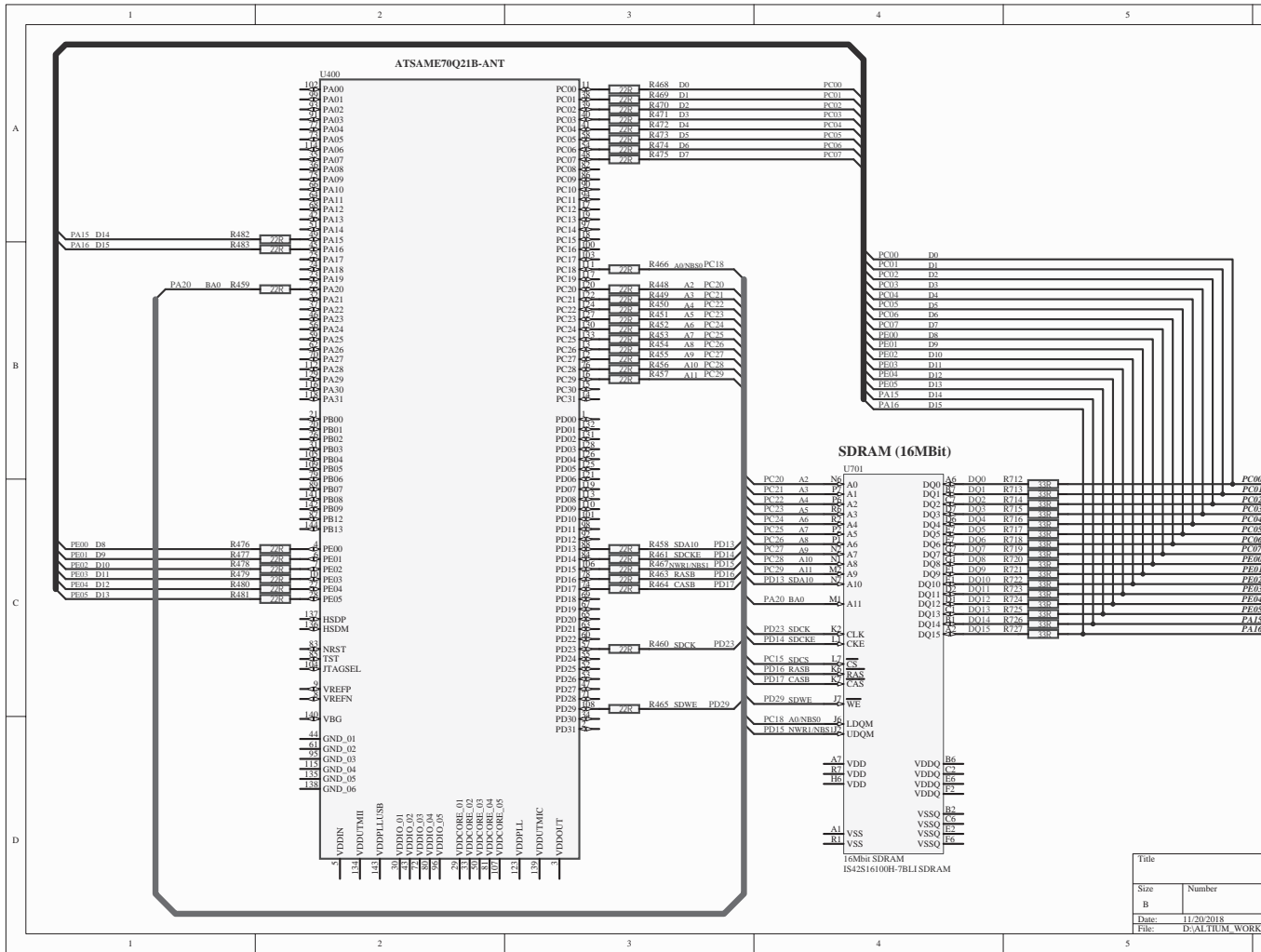
Figure 60-3. Schematic Example with a 16 Mb/16-bit SDRAM
