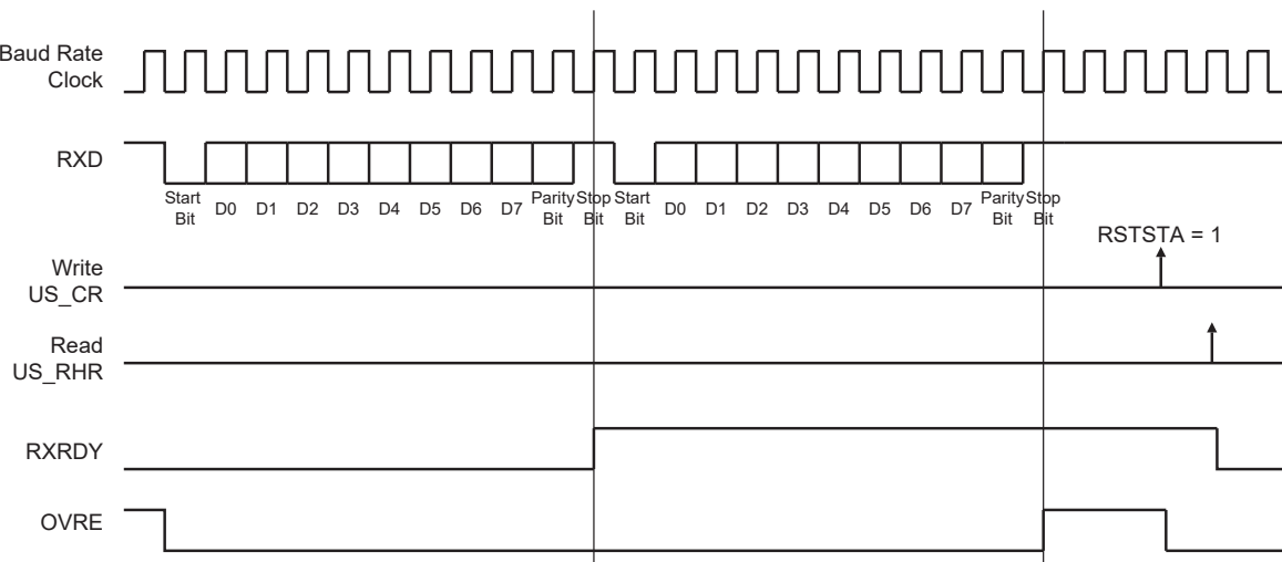
Figure 46-20. Receiver Status
