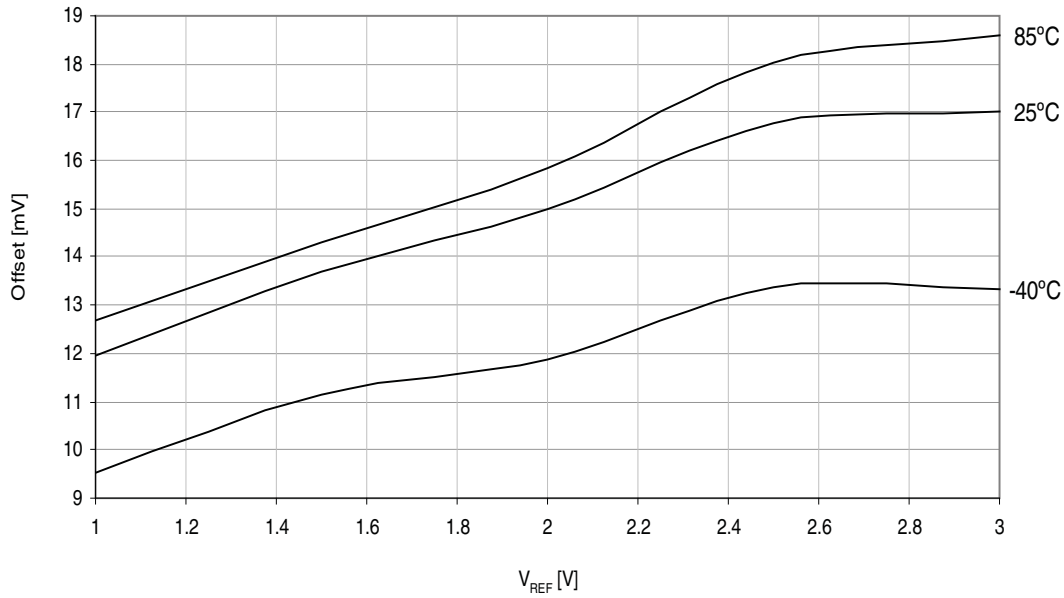
Figure 37-30. ADC Offset vs. V_{REF} Differential signed mode, V_{CC} = 3.6V , external reference.
