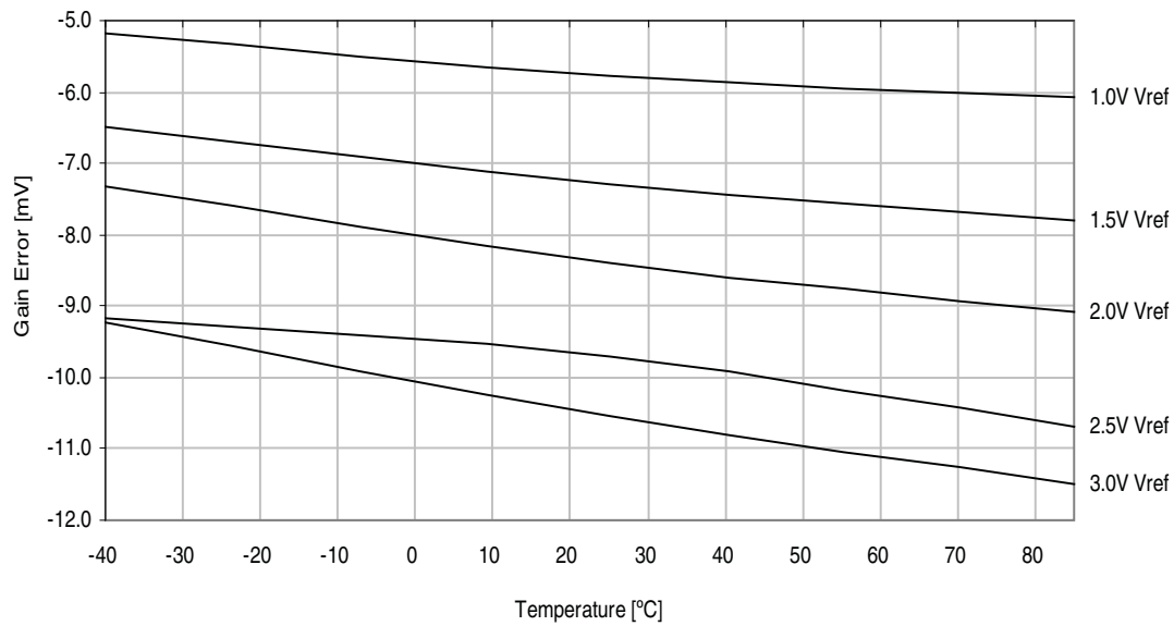
Figure 37-36. ADC Gain Error vs. Temperature. Differential signed mode, external reference.
