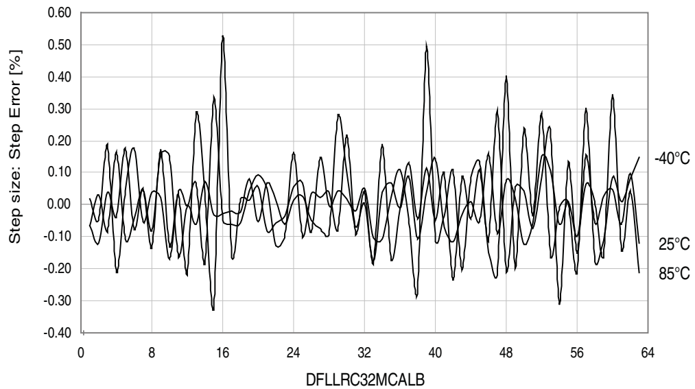
Figure 37-68. 32MHz internal oscillator CALB calibration step size.
