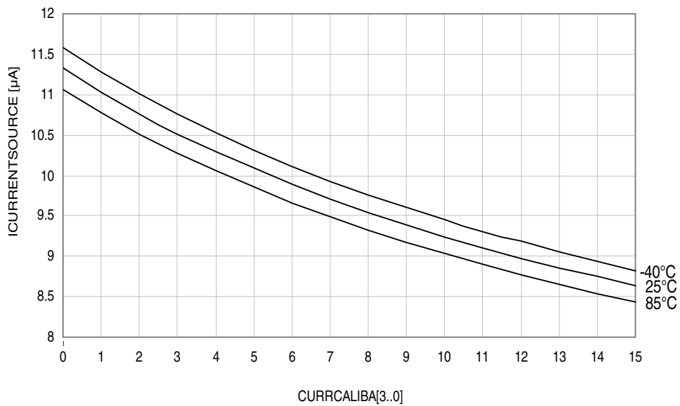
Figure 37-44. Analog comparator current source vs. Calibration.
