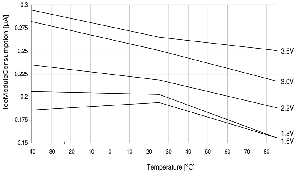
Figure 37-83. Psave vs. Temperature RTC, WDT, BOD sampled.
