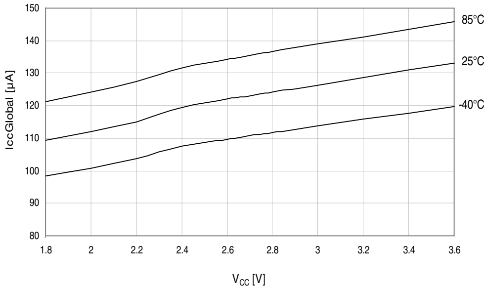
Figure 37-46.BOD current consumption vs. V_{CC} . Continuous mode, BOD level = 1.6V.
