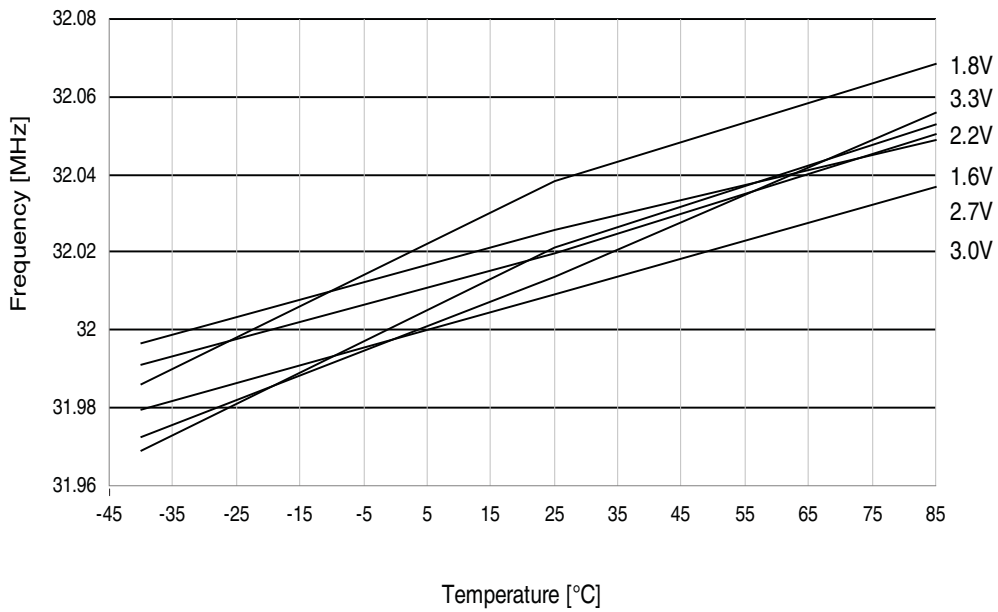
Figure 37-66. 32MHz internal oscillator frequency vs. temperature.
