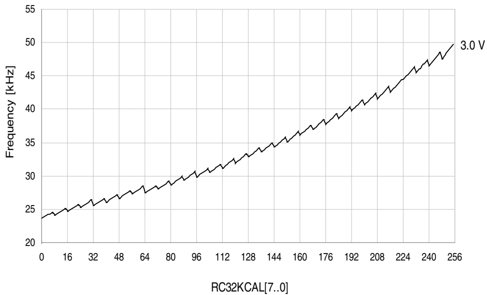
Figure 37-60. 32.768kHz internal oscillator frequency vs. calibration value.
