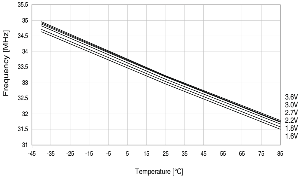
Figure 37-66. 32MHz internal oscillator frequency vs. temperature.
