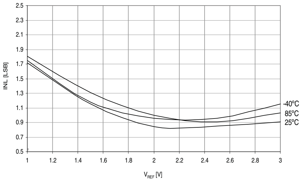
Figure 37-24. ADC INL vs. V_{REF} . Differential signed mode, V_{CC} = 3.6V , external reference.
