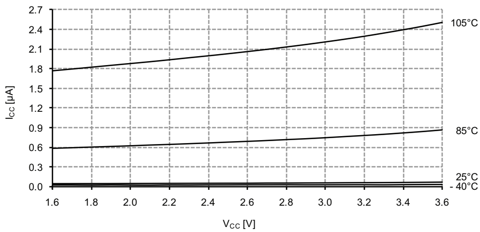
Figure 37-184. Power-down mode supply current vs. V_{CC} . All functions disabled.
