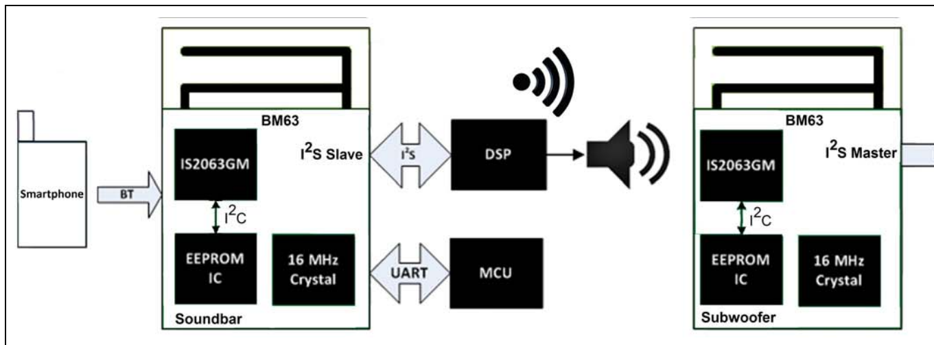
FIGURE 1-3: SOUNDBAR AND SUBWOOFER APPLICATIONS USING BM63 MODULE AND SMARTPHONE
