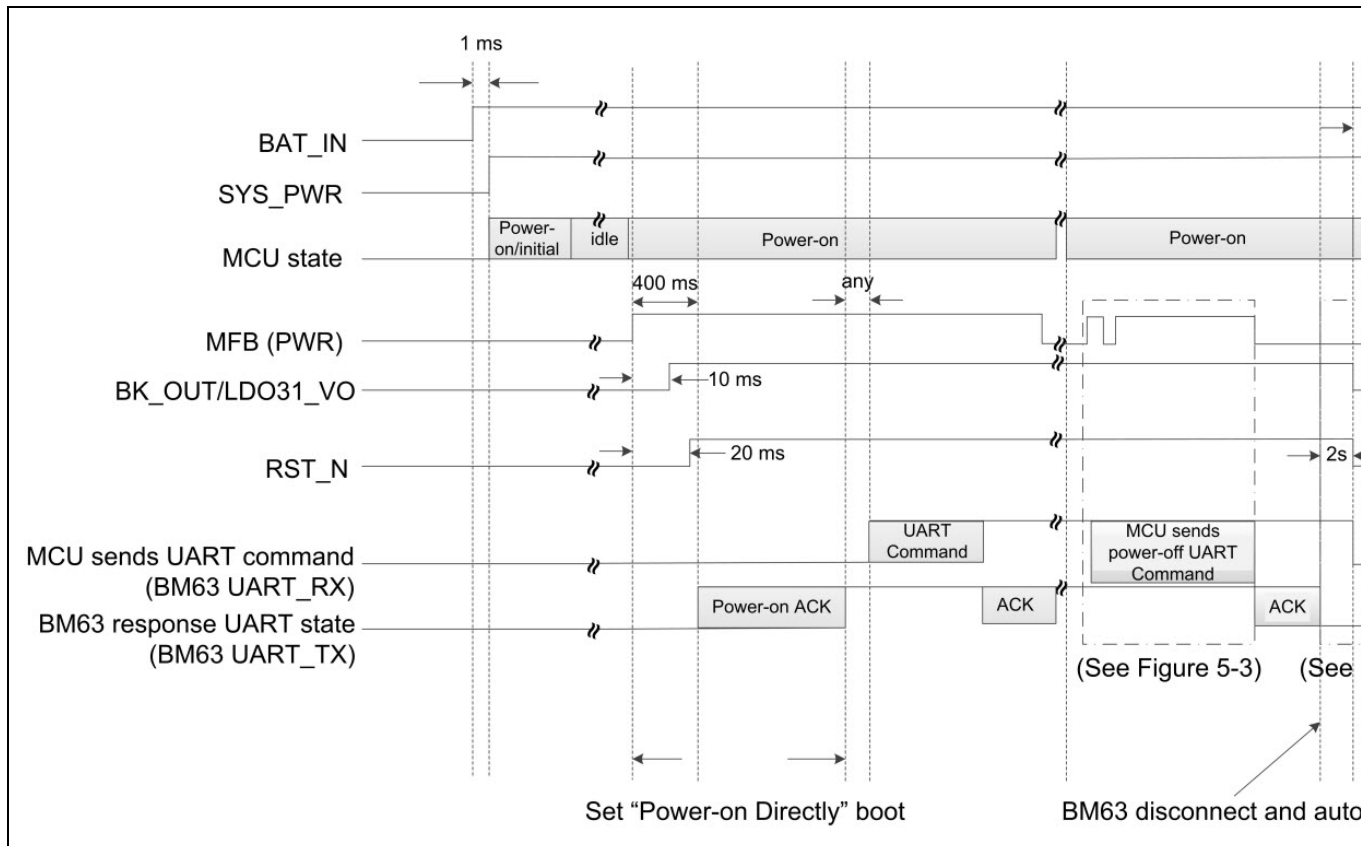
FIGURE 5-2: POWER-ON/OFF SEQUENCE
