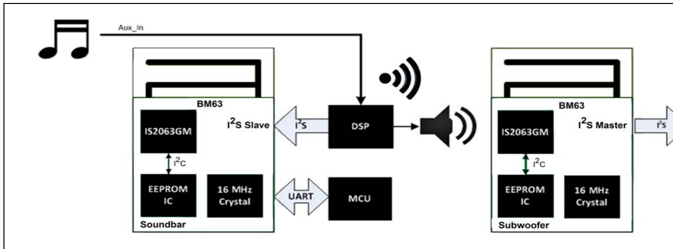
FIGURE 1-2: SOUNDBAR AND SUBWOOFER APPLICATIONS USING BM63 MODULE
