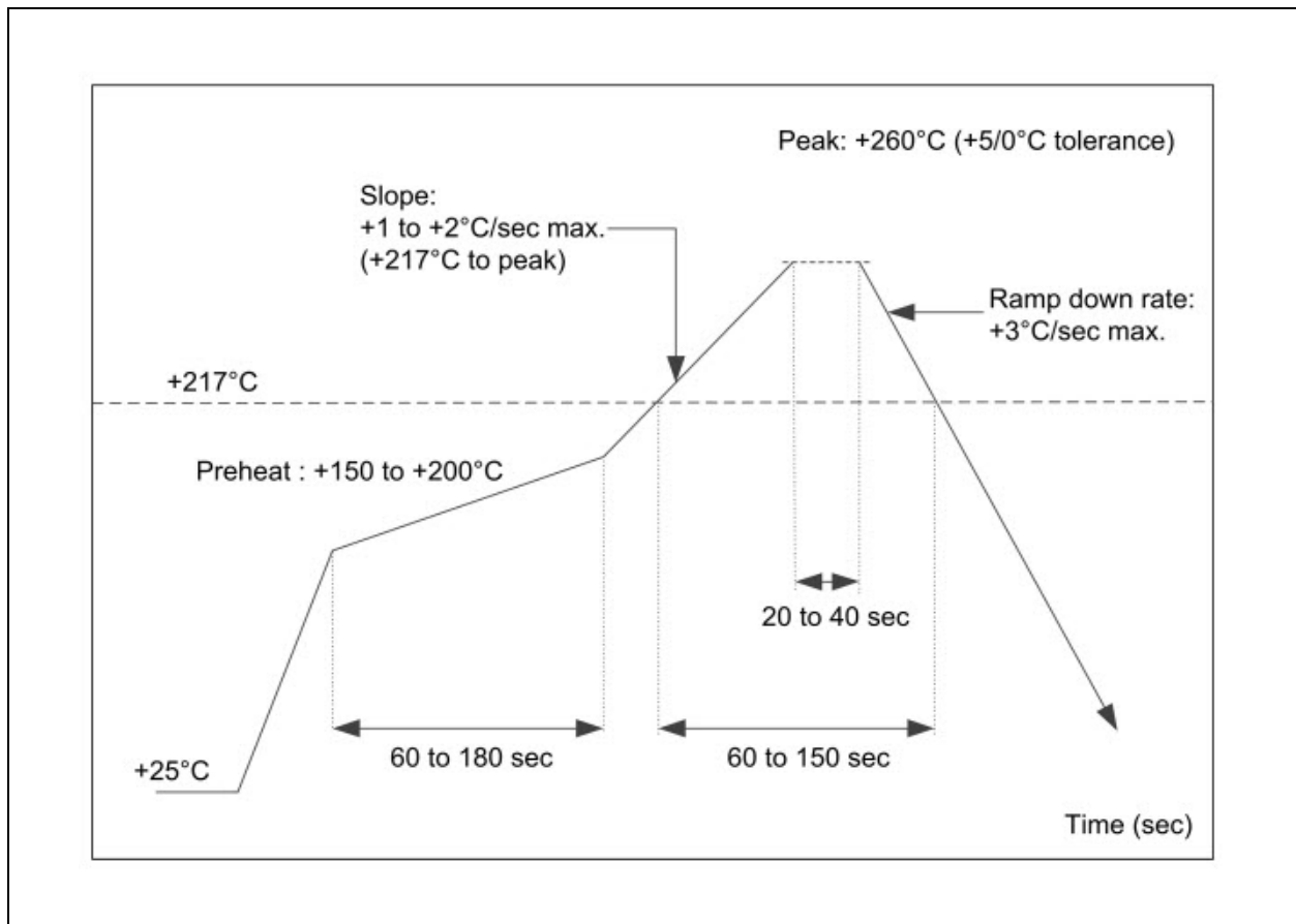
FIGURE 9-1: REFLOW PROFILE
