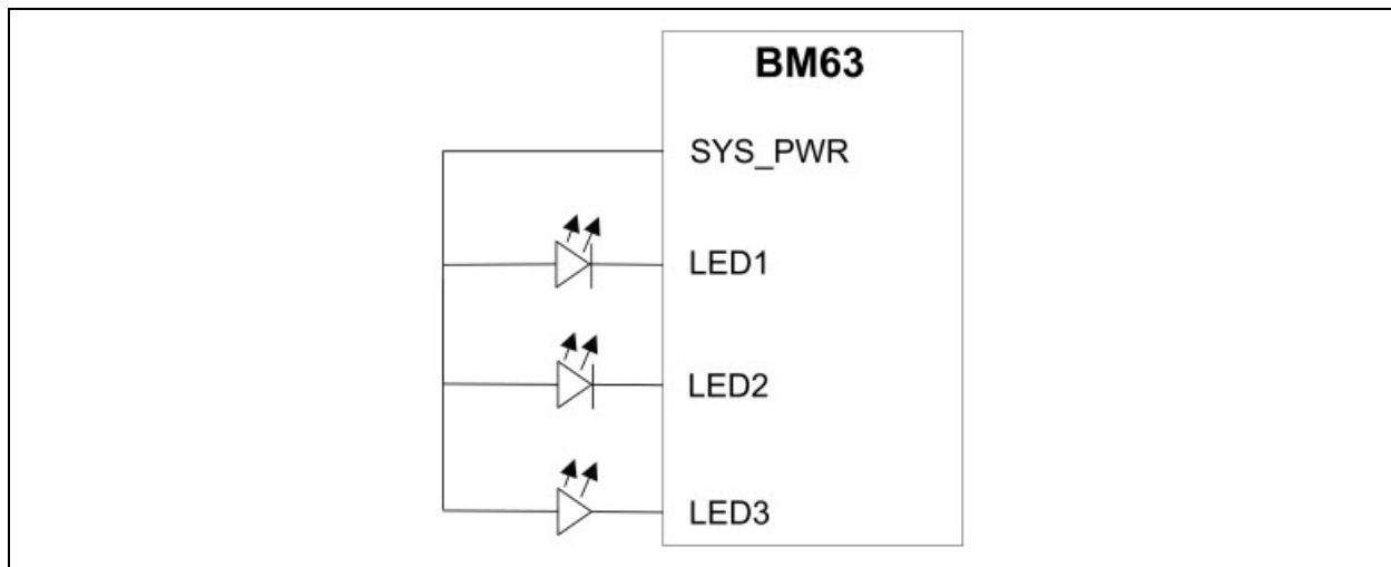
FIGURE 4-2: LED DRIVER
