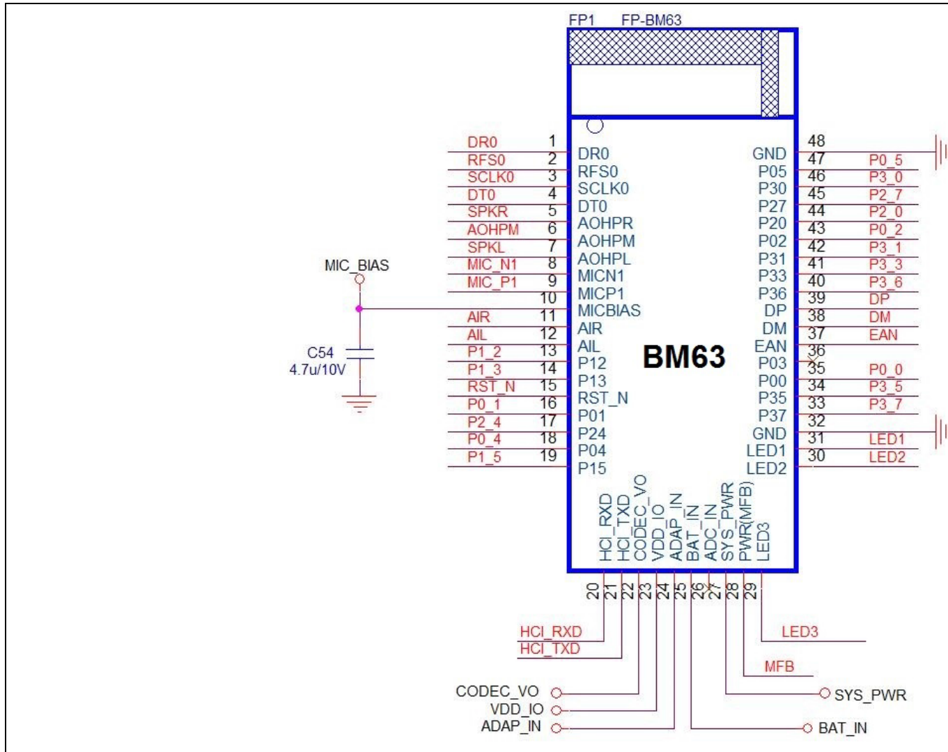
FIGURE 5-10: BM63 REFERENCE CIRCUIT FOR STEREO HEADSET APPLICATIONS
