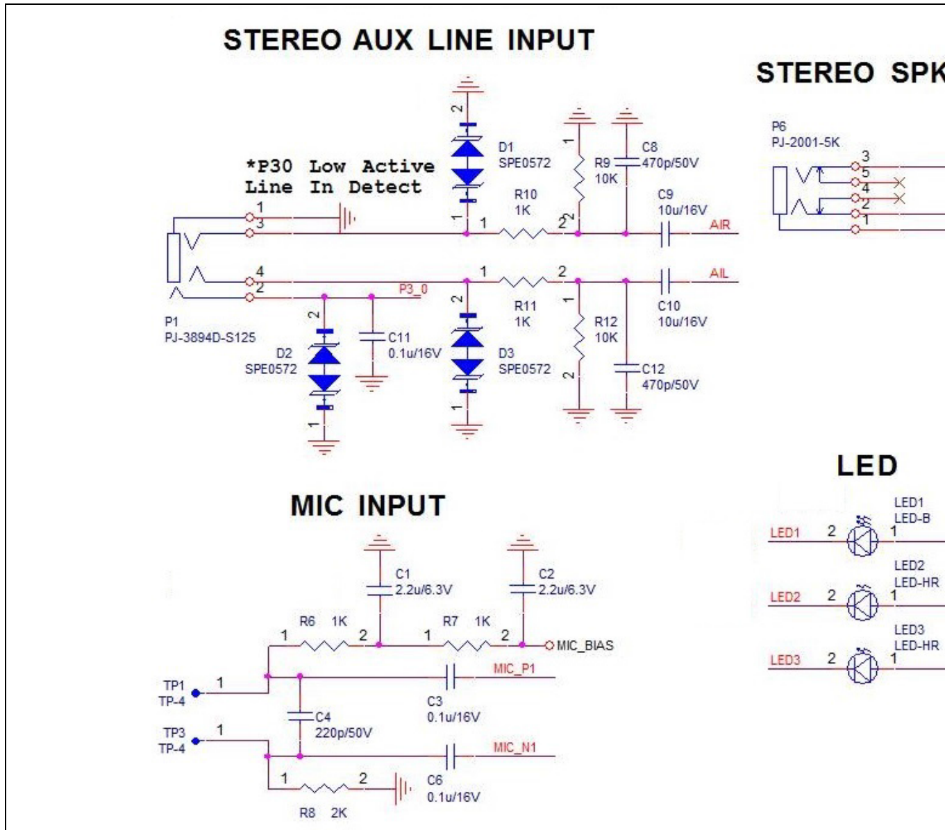
FIGURE 5-12: BM63 REFERENCE CIRCUIT FOR STEREO HEADSET APPLICATIONS
