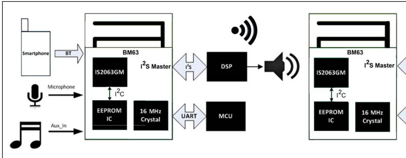
FIGURE 1-4: MULTI-SPEAKER APPLICATION USING BM63 MODULE
