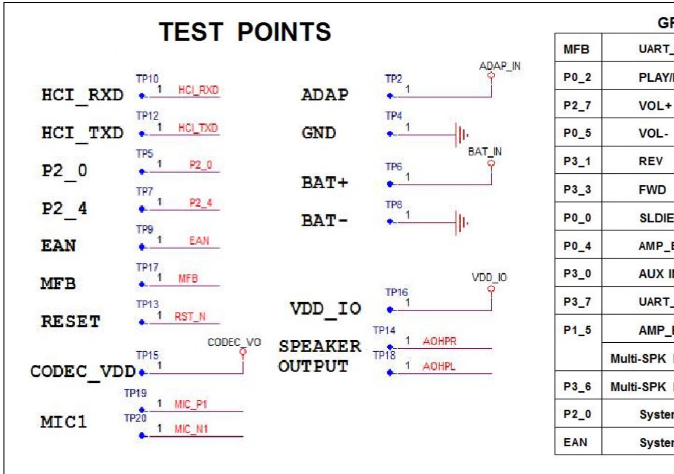
FIGURE 5-11: BM63 REFERENCE CIRCUIT FOR STEREO HEADSET APPLICATIONS
