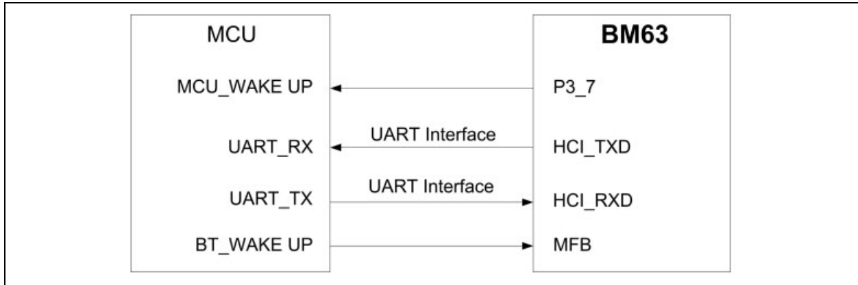
FIGURE 5-1: HOST MCU INTERFACE OVER UART
