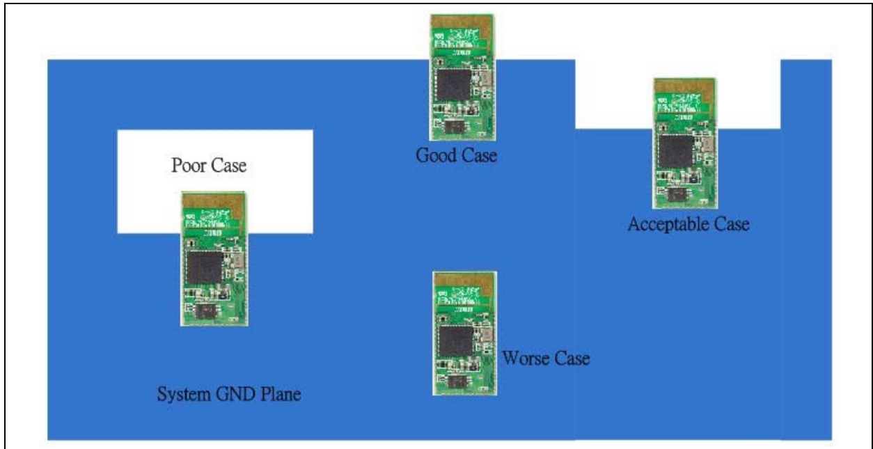
FIGURE 6-4: GND PLANE ON MAIN APPLICATION BOARD
