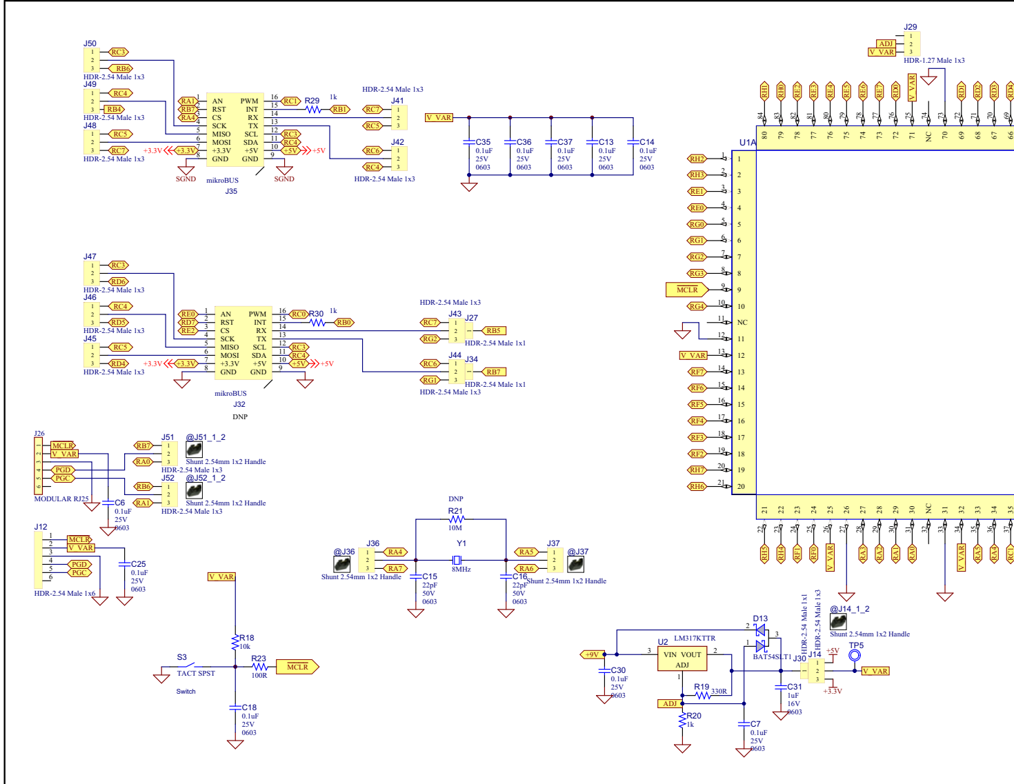
FIGURE A-3: EXPLORER 8 DEVELOPMENT SCHEMATIC - 2
