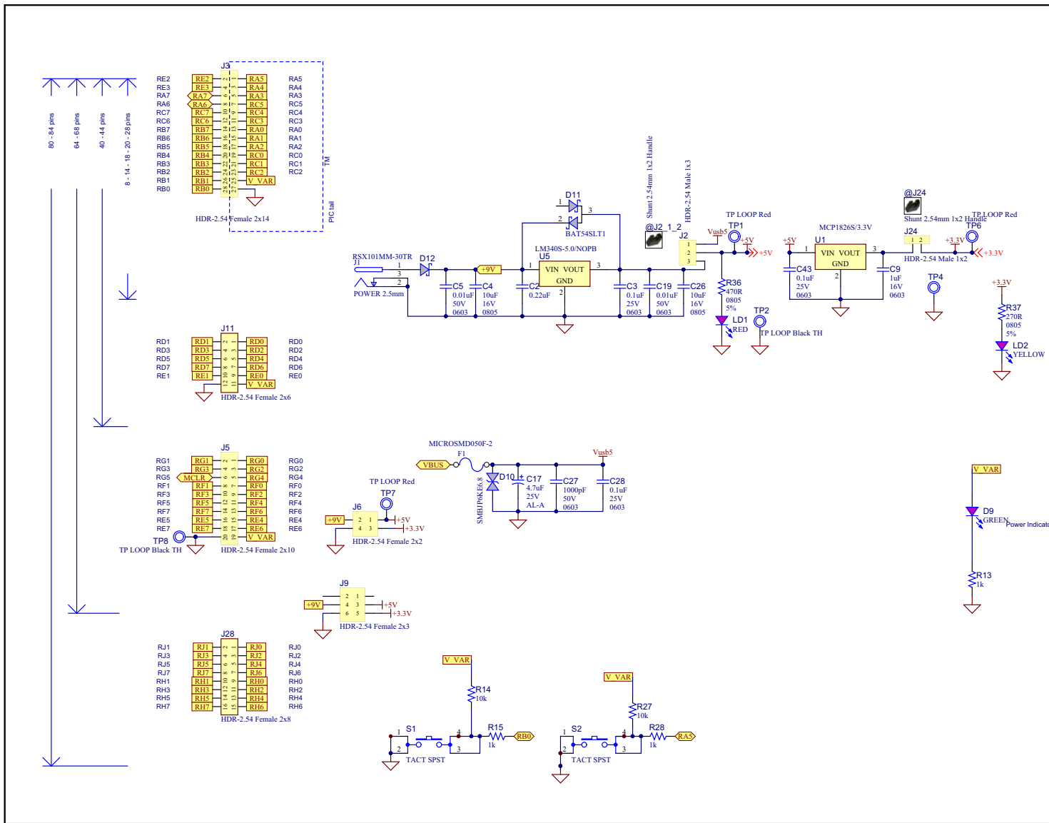
FIGURE A-2: EXPLORER 8 DEVELOPMENT SCHEMATIC - 1
