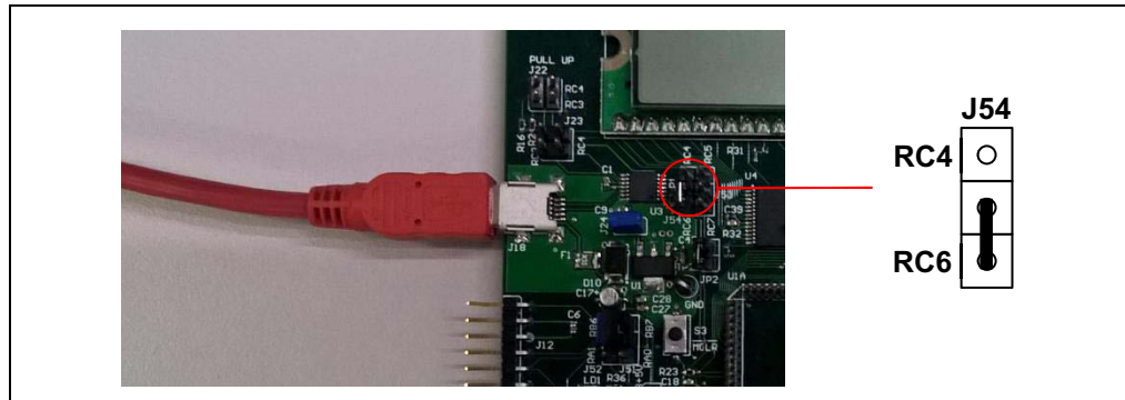
FIGURE 2-5: SETUP FOR UART TRANSMIT MODE
