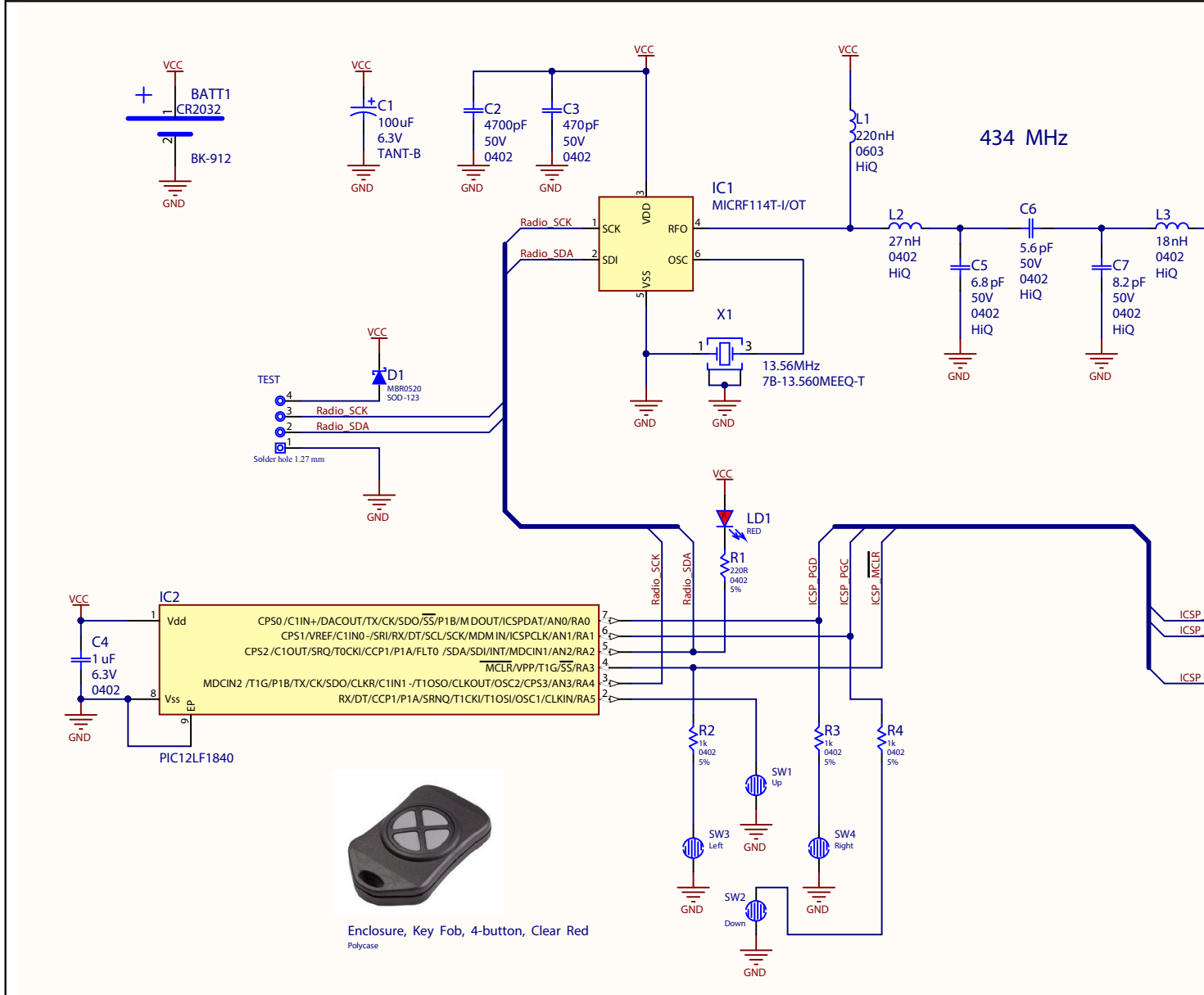
FIGURE A-5: MICRF114 WIRELESS REMOTE KEY FOB SCHEMATIC
