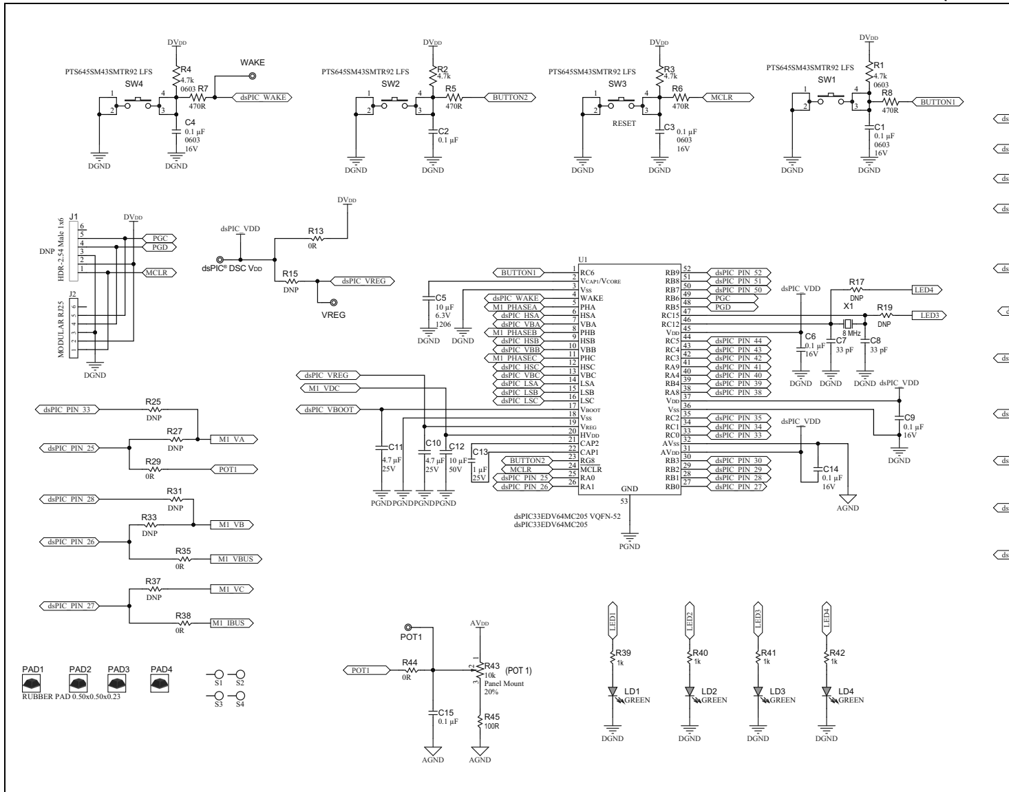
FIGURE A-1: dsPIC33EDV64MC205 MOTOR CONTROL DEVELOPMENT BOARD SCHEMATIC REV. 1.0 (SHEET
