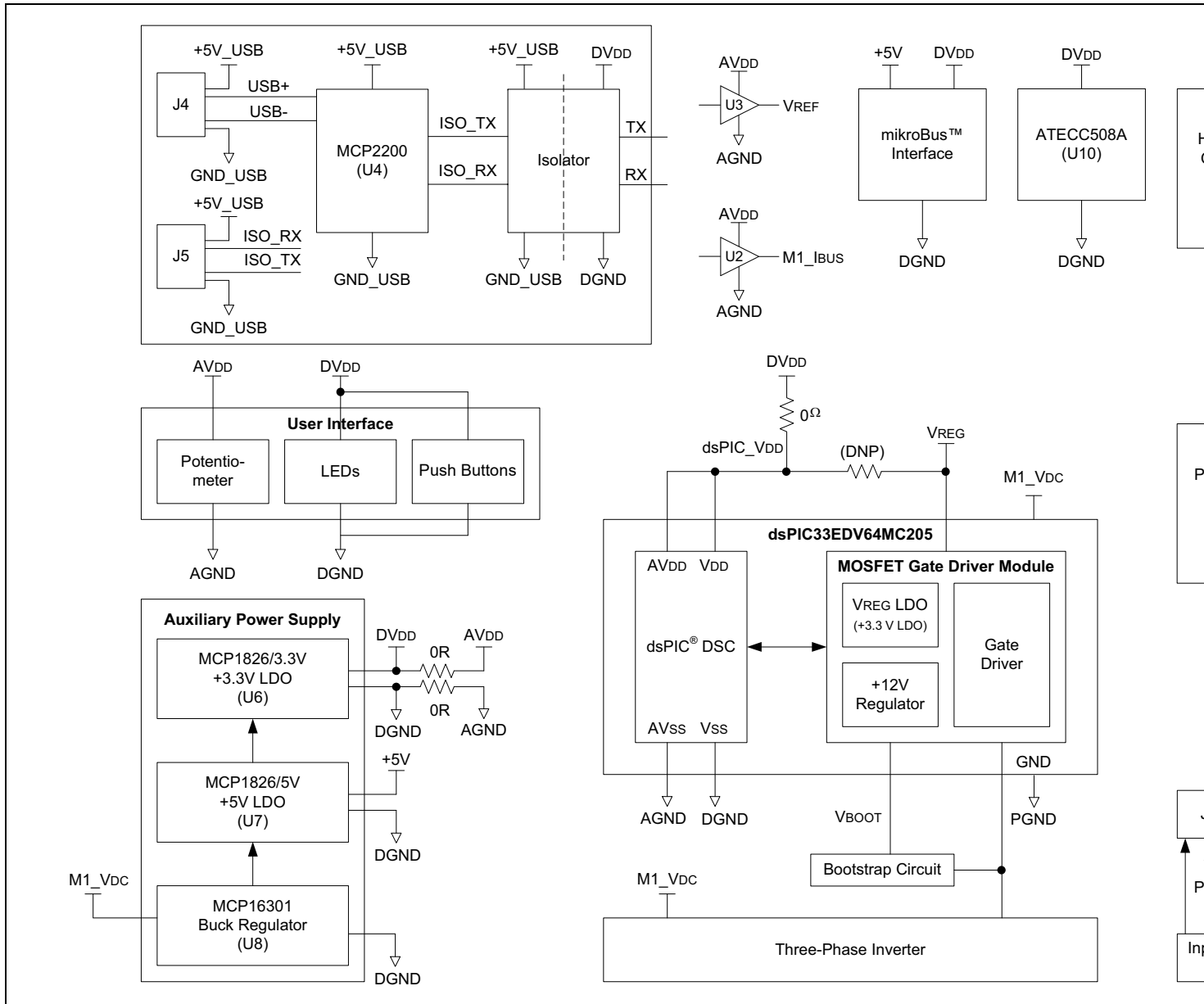
FIGURE 3-3: DEVELOPMENT BOARD POWER SUPPLY INTERCONNECTIONS
