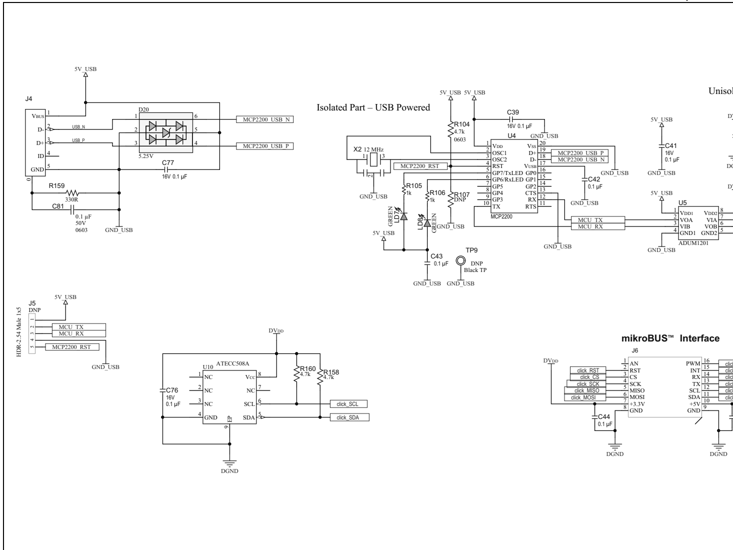
FIGURE A-5: dsPIC33EDV64MC205 MOTOR CONTROL DEVELOPMENT BOARD SCHEMATIC REV. 1.0 (SHEET 1)
