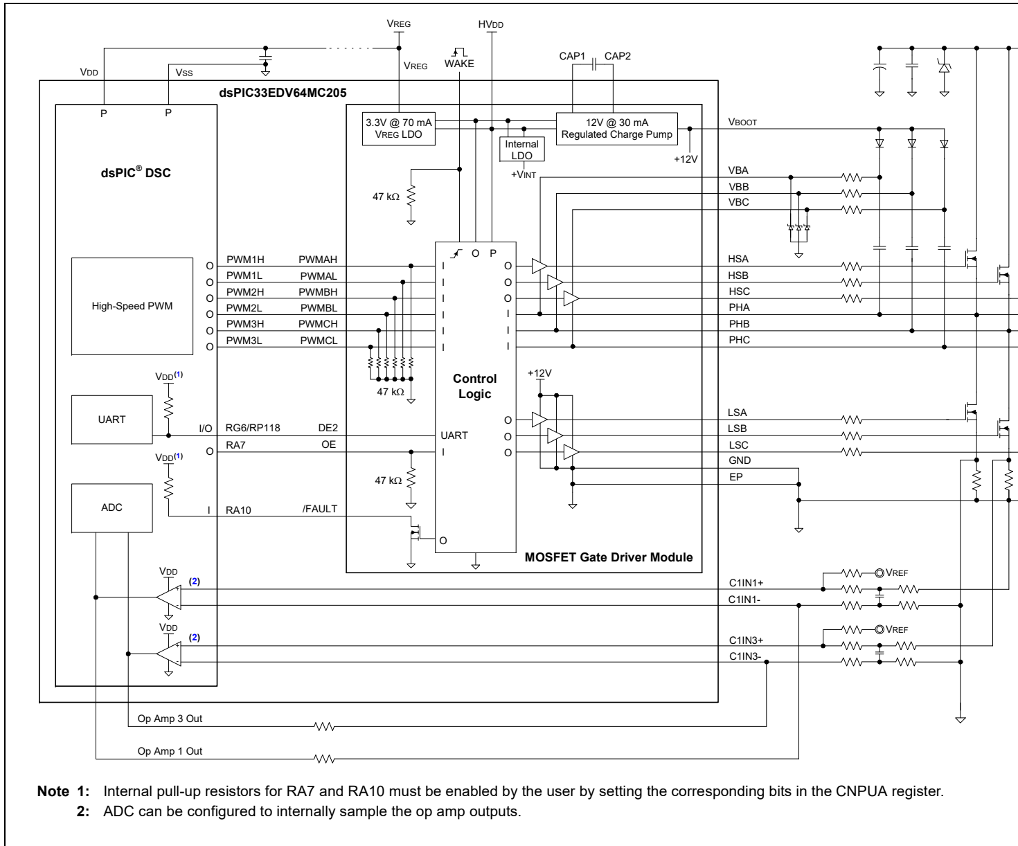
FIGURE 3-2: dsPIC33EDV64MC205 AND RELATED CIRCUITS
