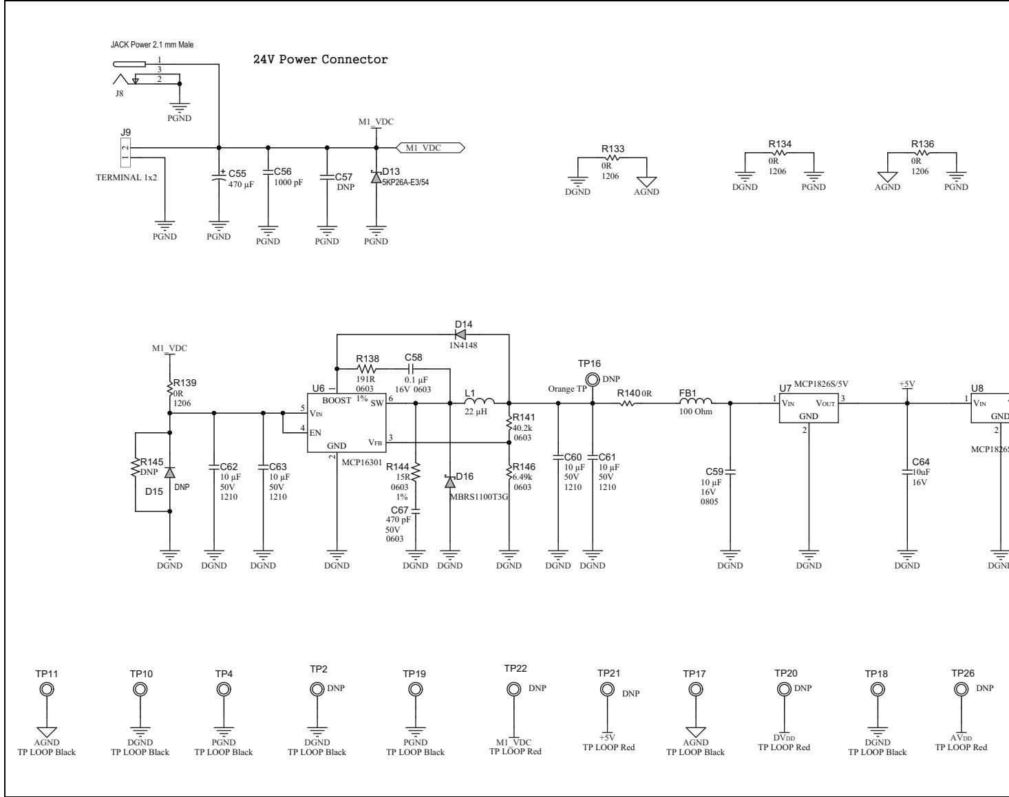
FIGURE A-4: dsPIC33EDV64MC205 MOTOR CONTROL DEVELOPMENT BOARD SCHEMATIC REV. 1.0 (SHEET
