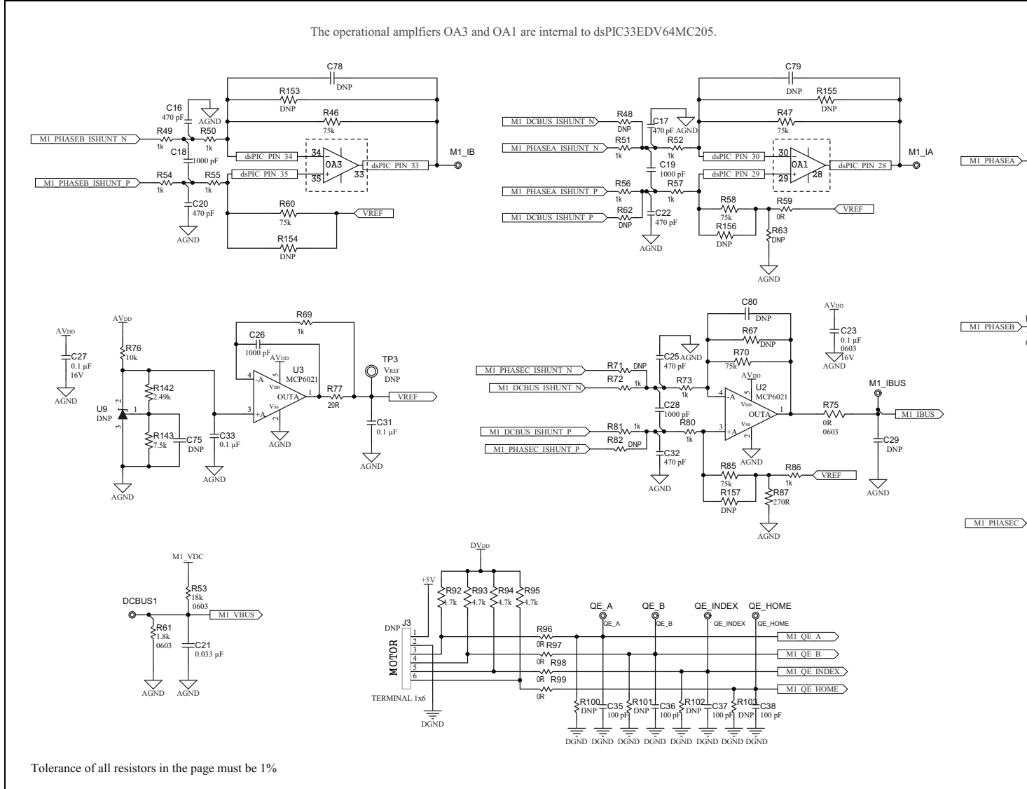
FIGURE A-2: dsPIC33EDV64MC205 MOTOR CONTROL DEVELOPMENT BOARD SCHEMATIC REV. 1.0 (SHEET
