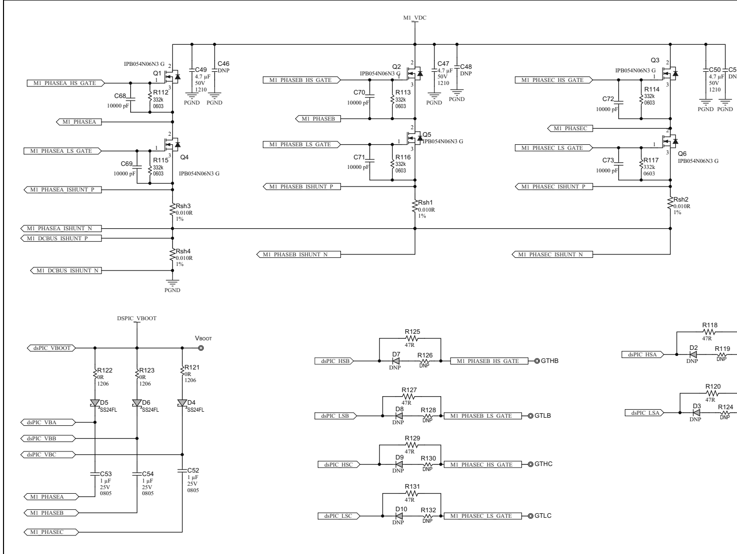
FIGURE A-3: dsPIC33EDV64MC205 MOTOR CONTROL DEVELOPMENT BOARD SCHEMATIC REV. 1.0 (SHEET
