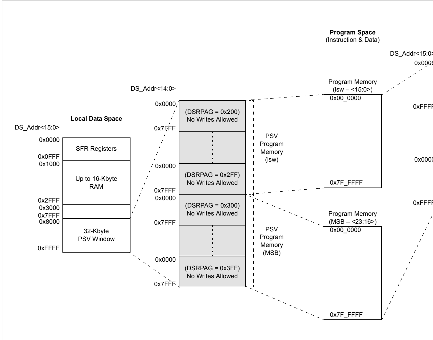
FIGURE 3-8: PAGED DATA MEMORY SPACE
