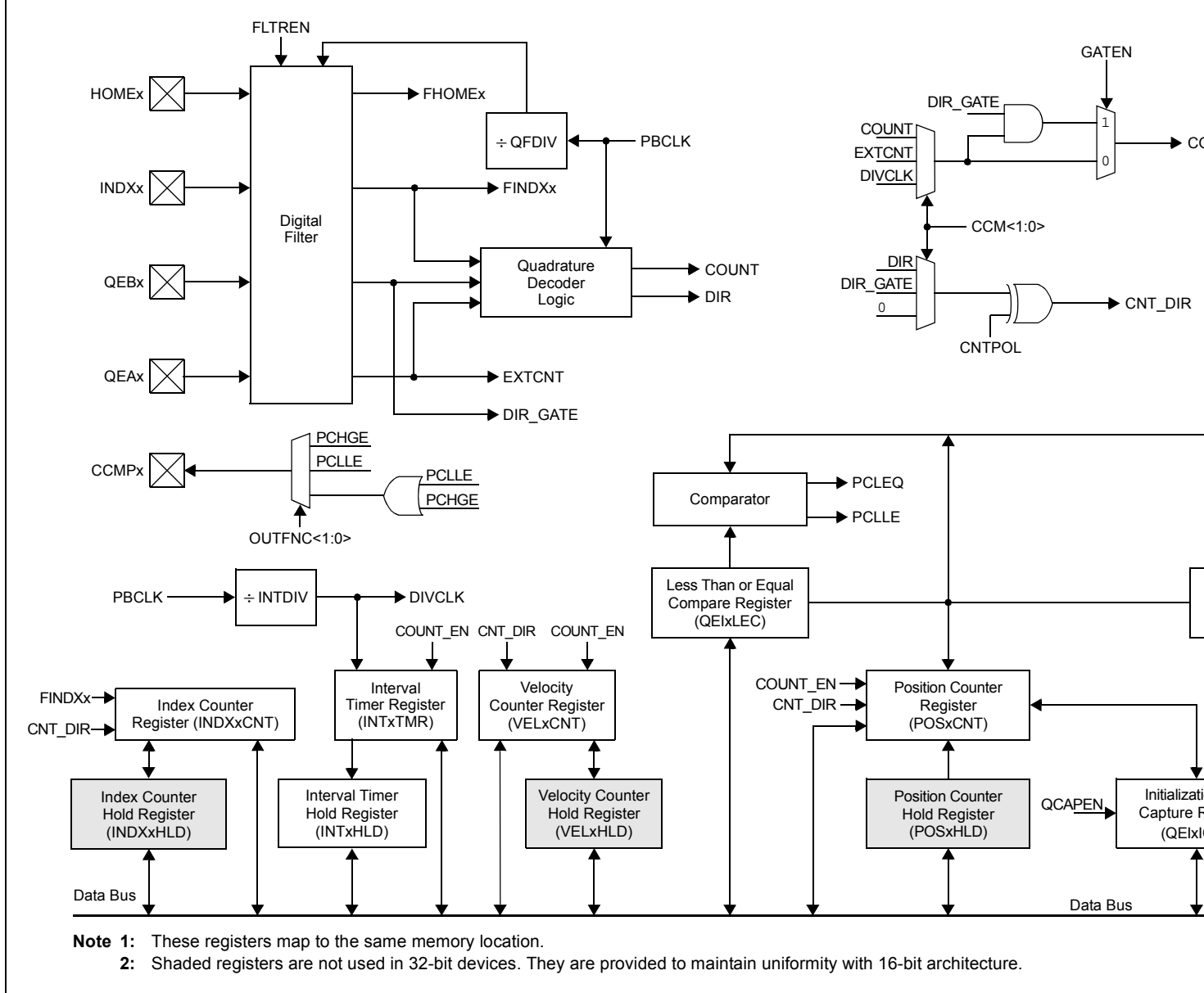
FIGURE 12-2: QUADRATURE ENCODER INTERFACE (QEI) MODULE BLOCK DIAGRAM
