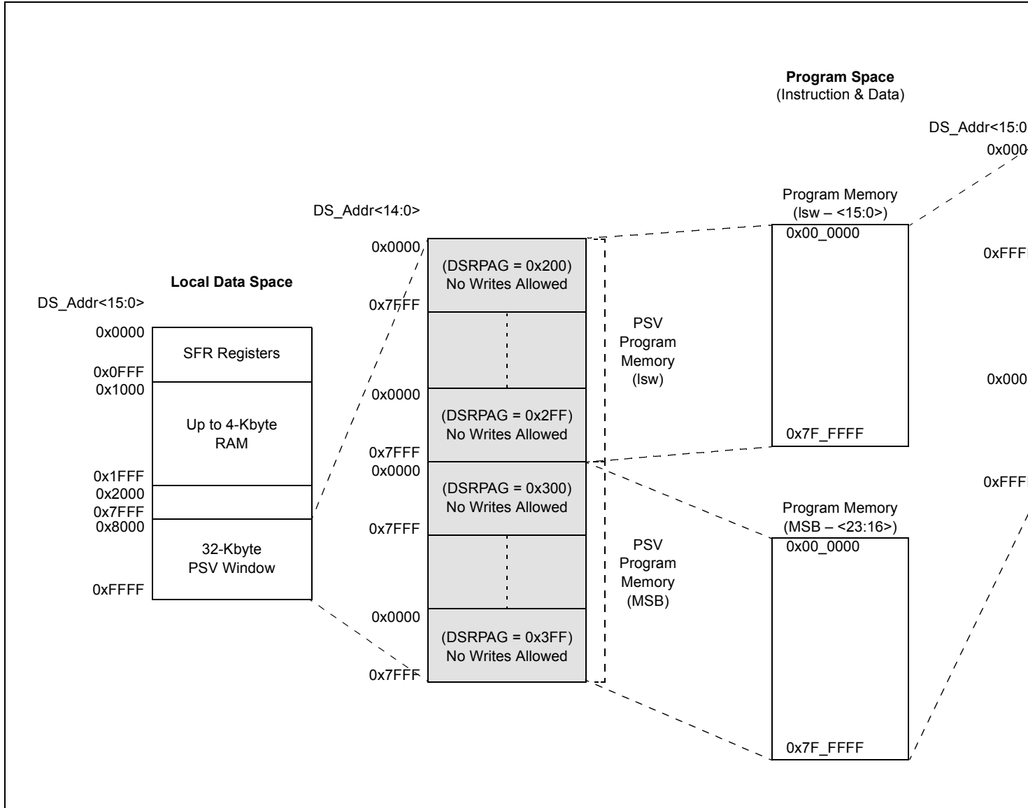
FIGURE 4-7: PAGED DATA MEMORY SPACE
