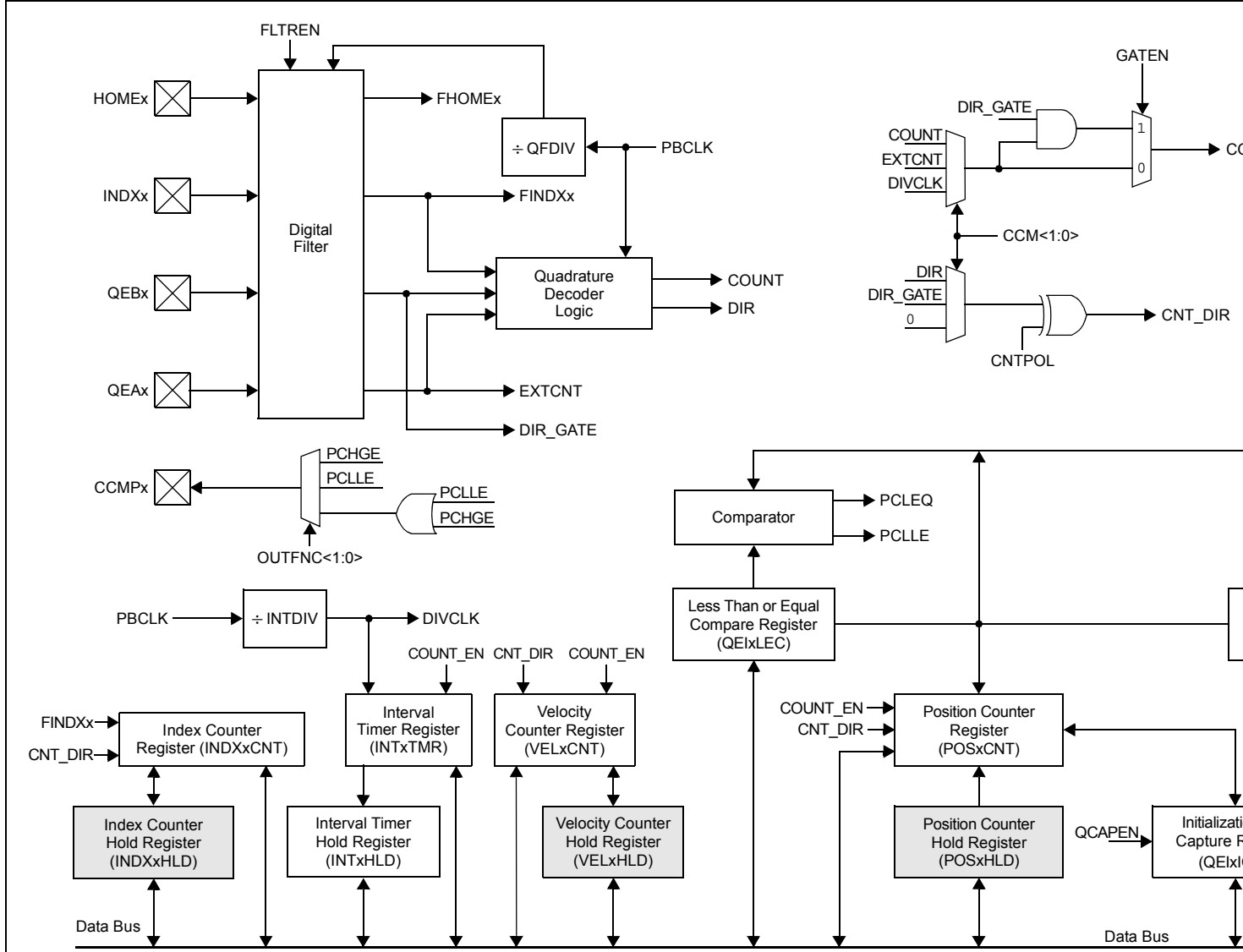
FIGURE 12-2: QUADRATURE ENCODER INTERFACE (QEI) MODULE BLOCK DIAGRAM
