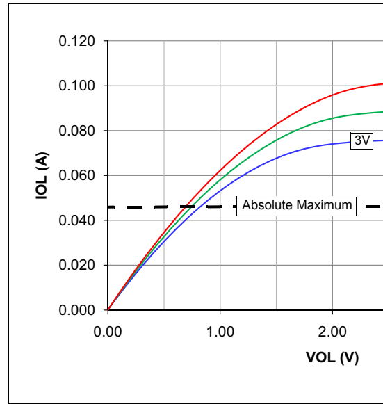
FIGURE 29-6: VOL – 16x DRIVER PINS
