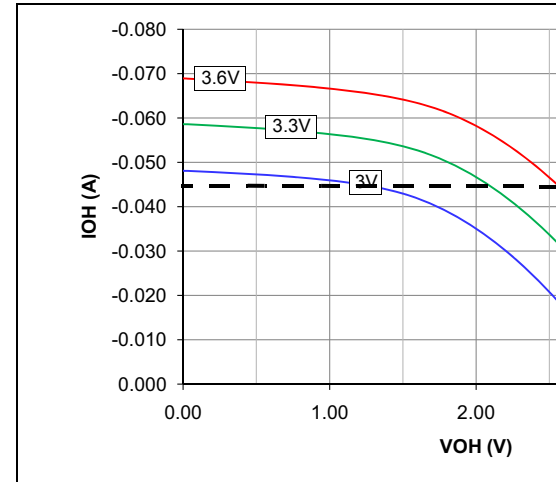
FIGURE 29-3: VOH – 16x DRIVER PINS
