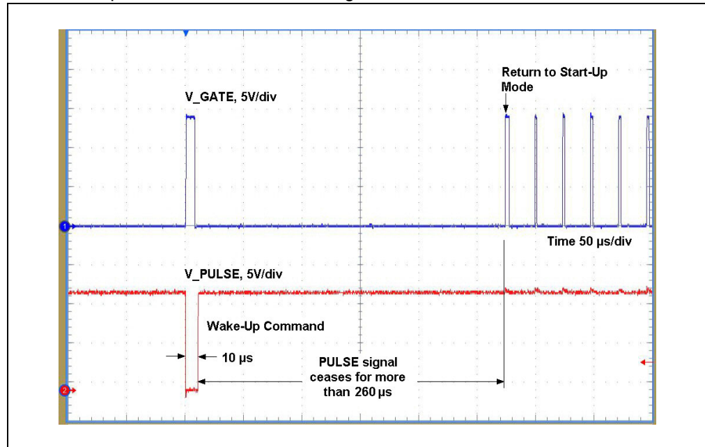
FIGURE 5-4: MCP1012 Wake-Up Command ( Figure 5-3 Detail).
