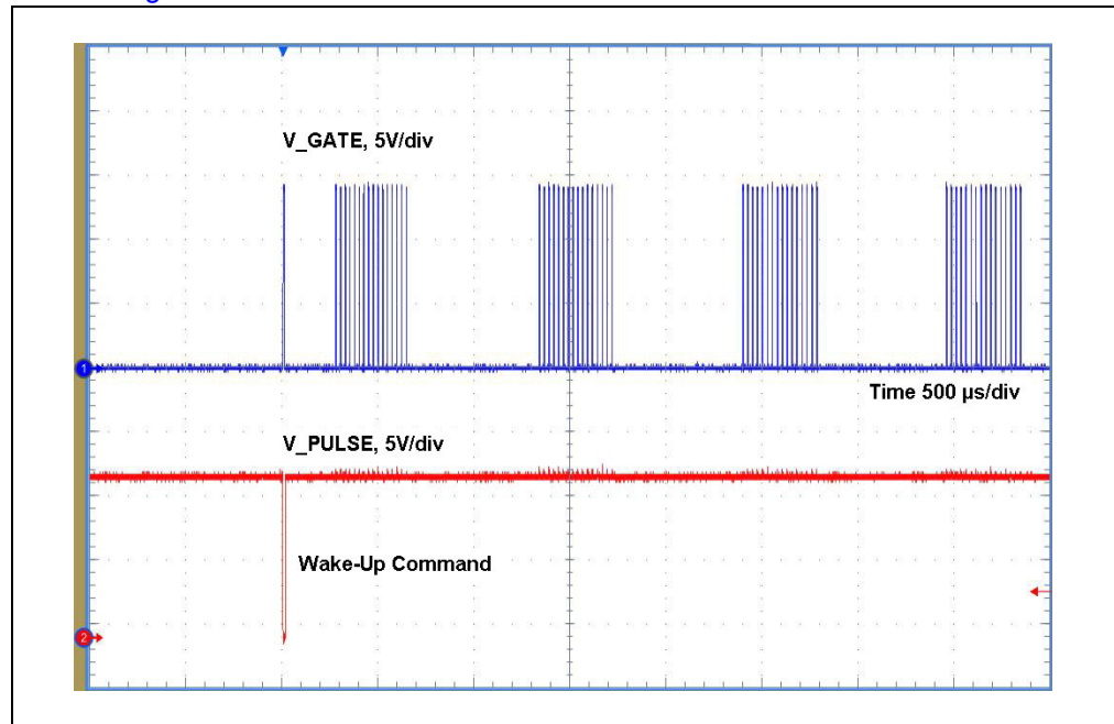
FIGURE 5-3: MCP1012 Wake-Up Command.
