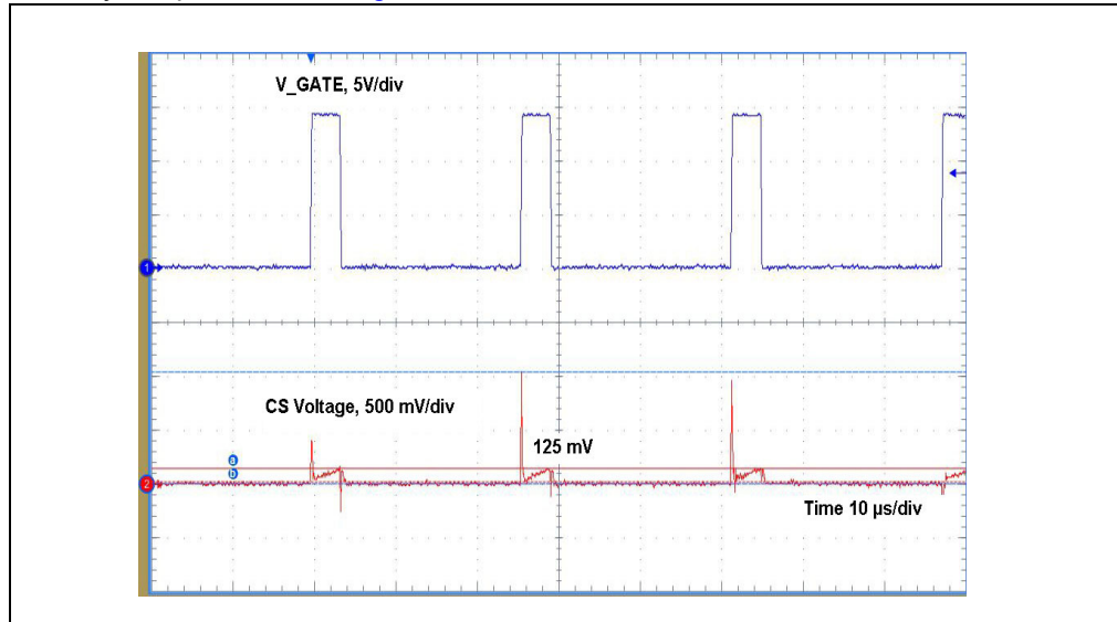
FIGURE 4-1: MCP1012 V_GATE and C/S Voltage.
