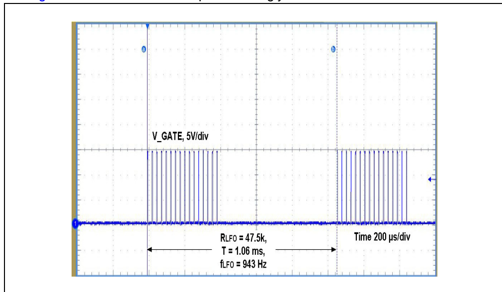
FIGURE 4-2: MCP1012 V_GATE Voltage.
