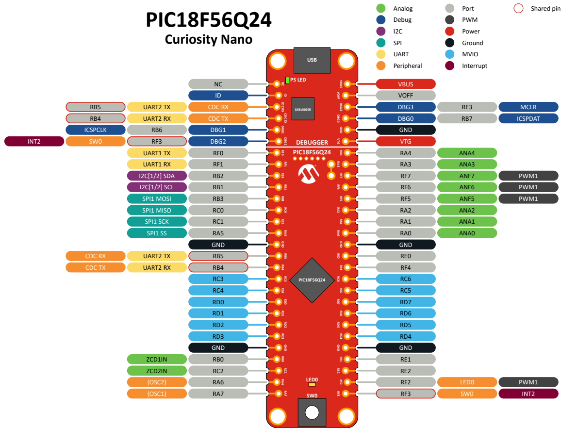
Figure 1-3. PIC18F56Q24 Curiosity Nano Pinout
