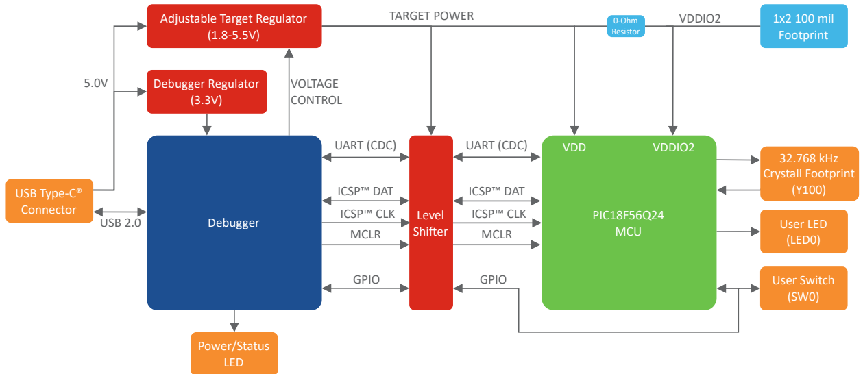
Figure 1-2. PIC18F56Q24 Curiosity Nano Board Block Diagram
