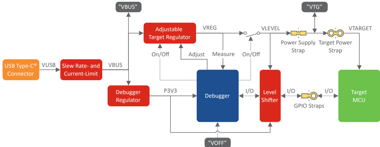
Figure 4-7. Power Supply Block Diagram
