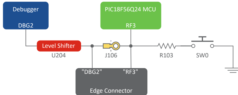
Figure 4-6. PIC18F56Q24 Curiosity Nano SW0 Block Diagram
