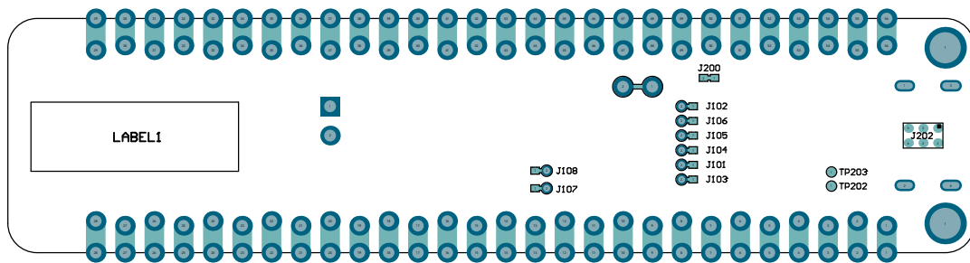
Figure 7-4. PIC18F56Q24 Curiosity Nano Assembly Drawing Bottom
