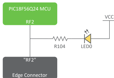
Figure 4-5. PIC18F56Q24 Curiosity Nano LED0 Block Diagram
