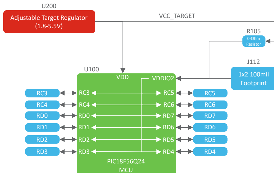
Figure 4-3. MVIO Block Diagram
