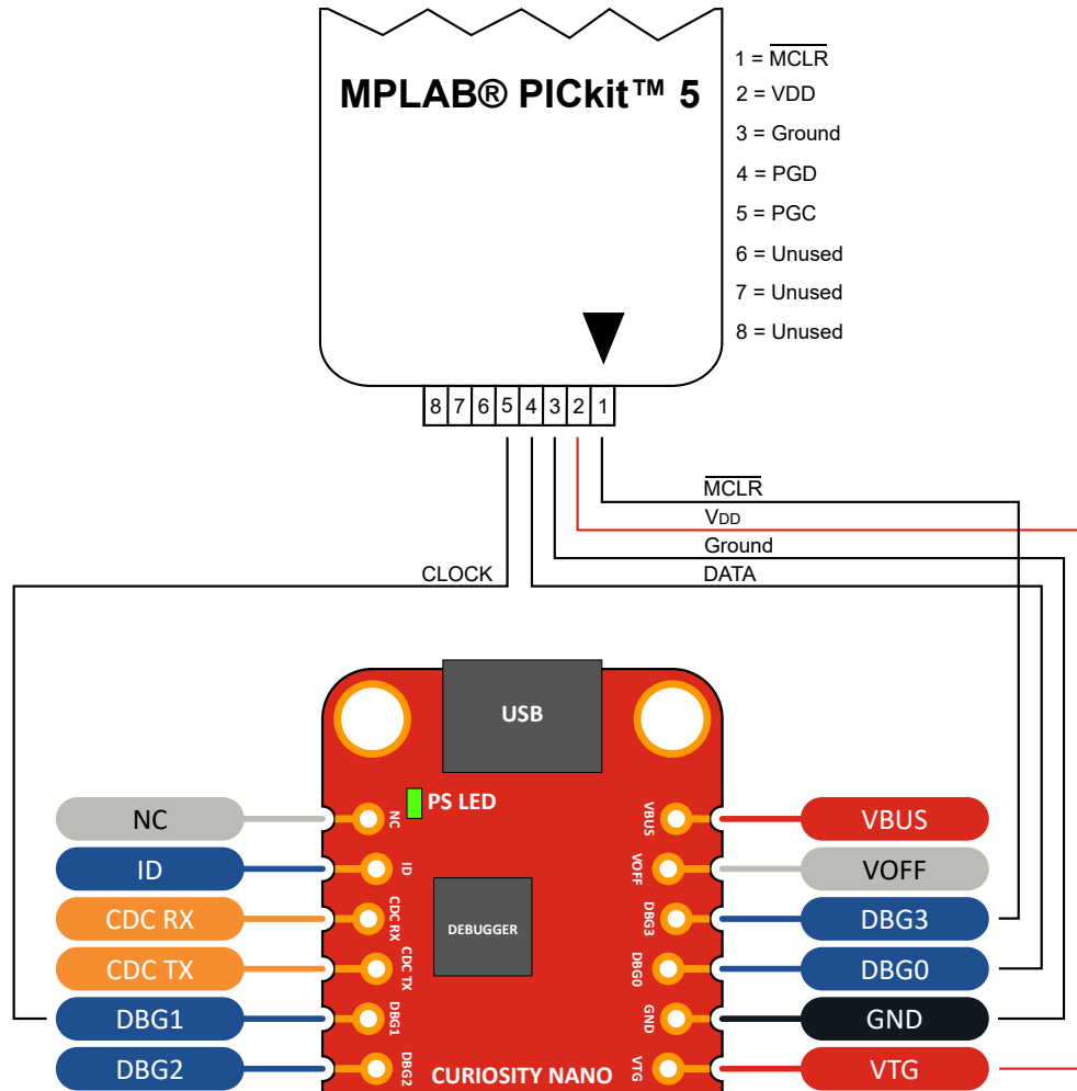
Figure 7-8. Connecting the MPLAB® PICKit™ 5 In-Circuit Debugger/Programmer to PIC18F56Q24 Curiosity Nano
