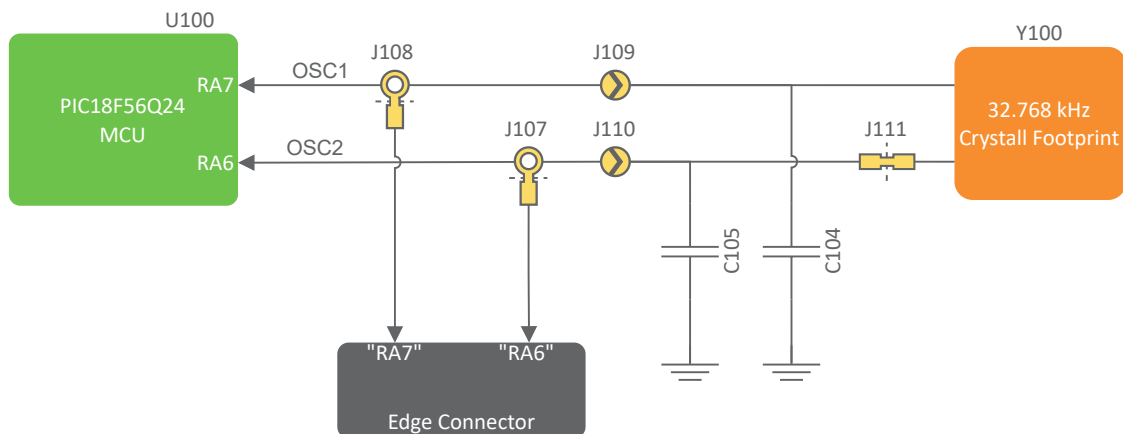
Figure 4-1. 32.768 kHz Crystal Block Diagram
