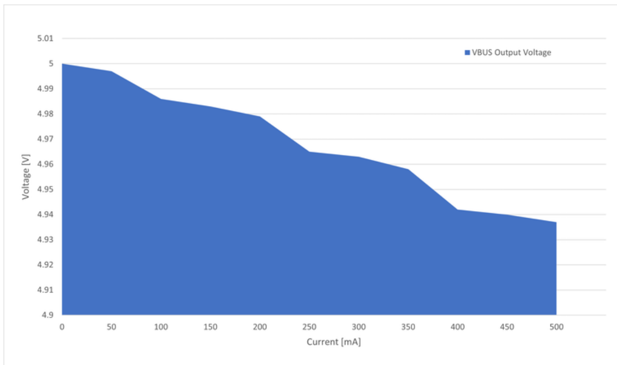
Figure 4-10. VBUS Output Voltage vs. Current
