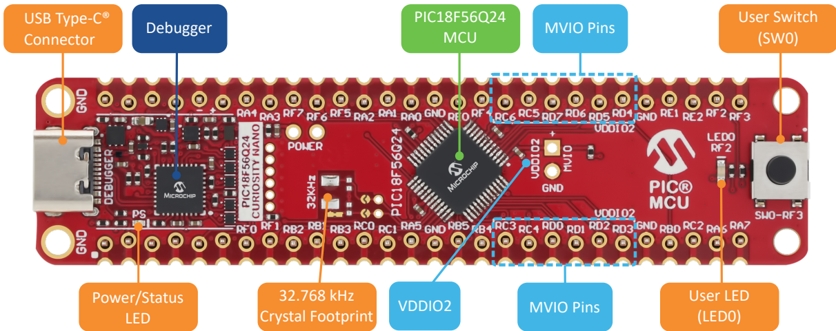
Figure 1-1. PIC18F56Q24 Curiosity Nano Board Overview
