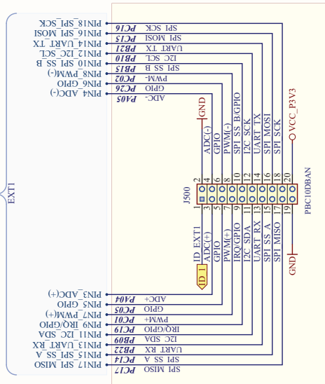
EXT1 Extension Header
