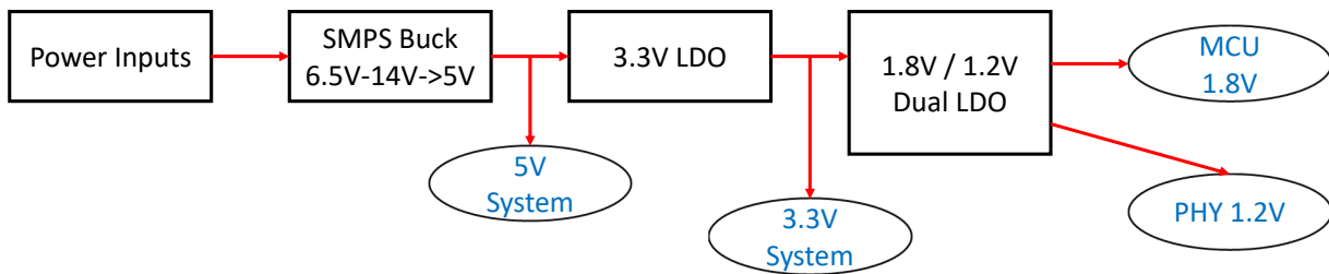
Figure 2-3. PIC32CK SG01/GC01 Curiosity Ultra Power Block Diagram
