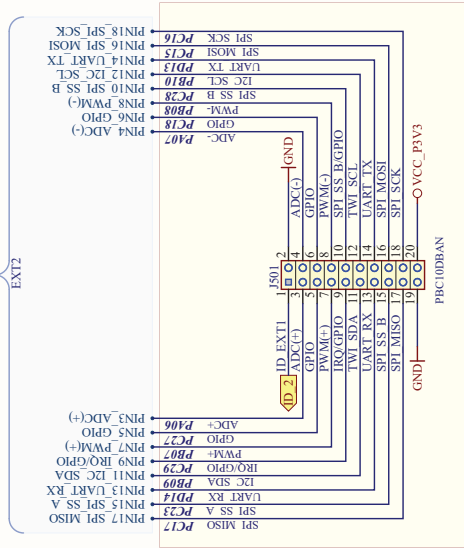
EXT2 Extension Header
