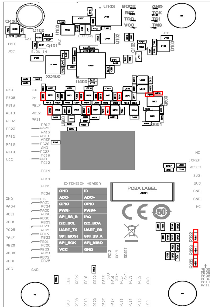
Figure 4-3. Resistors (Bottom View)
