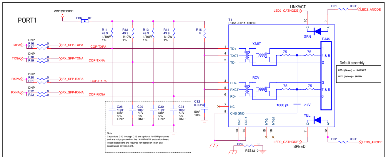
FIGURE B-4: EVB-LAN9355 EVALUATION BOARD SCHEMATIC 4
