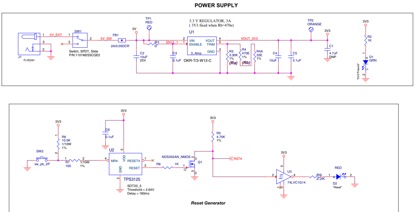
FIGURE B-2: EVB-LAN9355 EVALUATION BOARD SCHEMATIC 2
