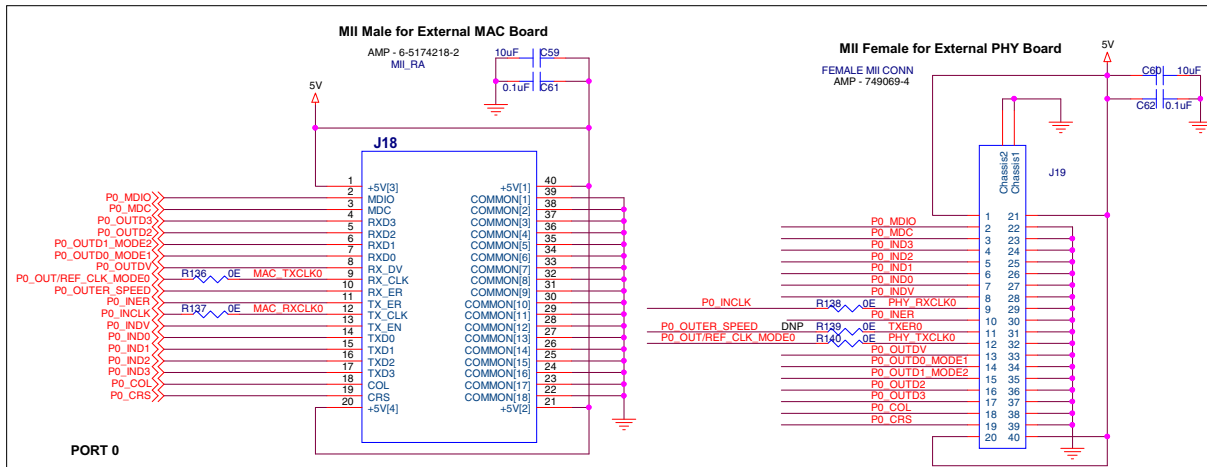
FIGURE B-8: EVB-LAN9355 EVALUATION BOARD SCHEMATIC 8
