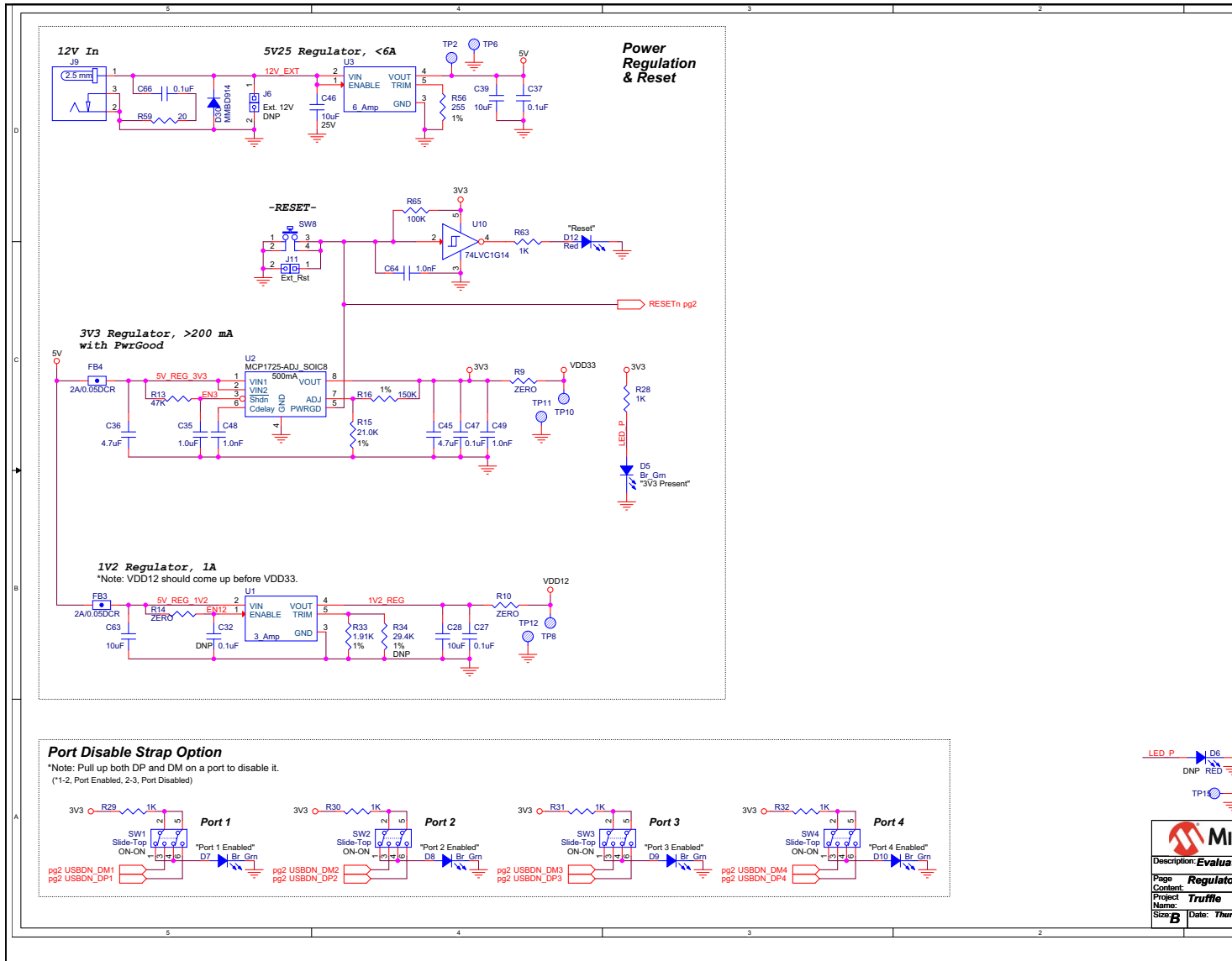
FIGURE B-2: EVB-USB5744 EVALUATION BOARD SCHEMATIC 2
