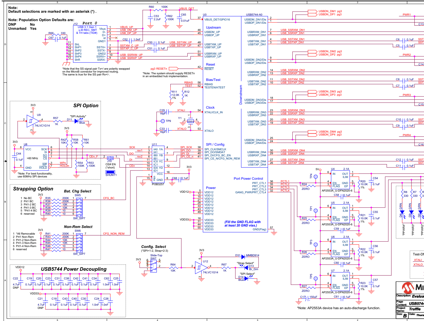
FIGURE B-1: EVB-USB5744 EVALUATION BOARD SCHEMATIC 1
