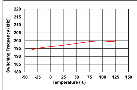
FIGURE 2-10: Switching Frequency vs. Temperature.
