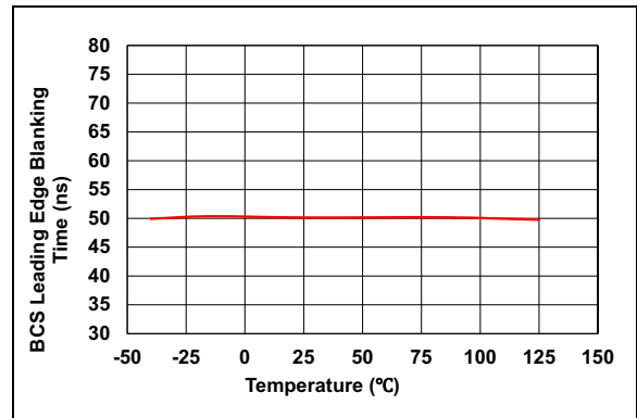
FIGURE 2-12: BCS Leading Edge Blanking Time vs. Temperature.
