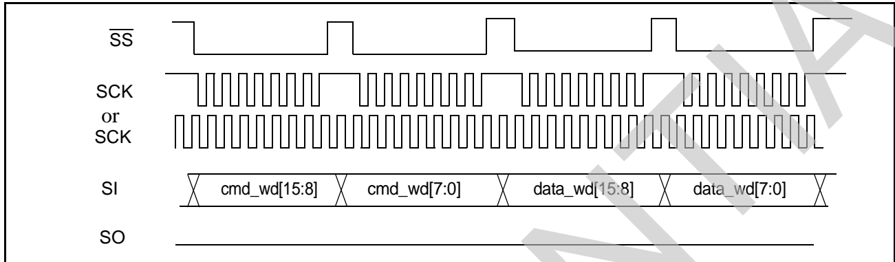
Figure 19 - One Data Word Write in Byte Framing Mode
