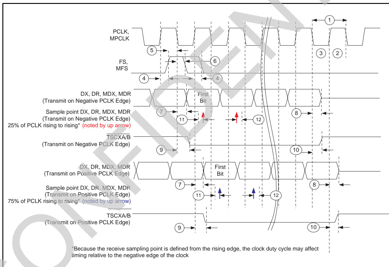
Figure 25 - PCM Highway Timing
