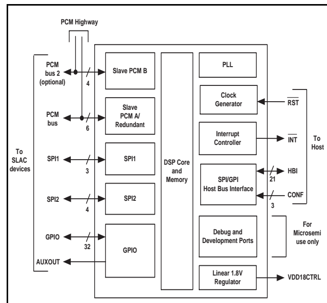
Figure 1 - Block Diagram
