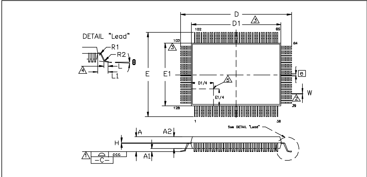
FIGURE 2: 128-PIN QPF PACKAGE, 14 X 20 X 2.7 BODY, 3.2MM FOOTPRINT
