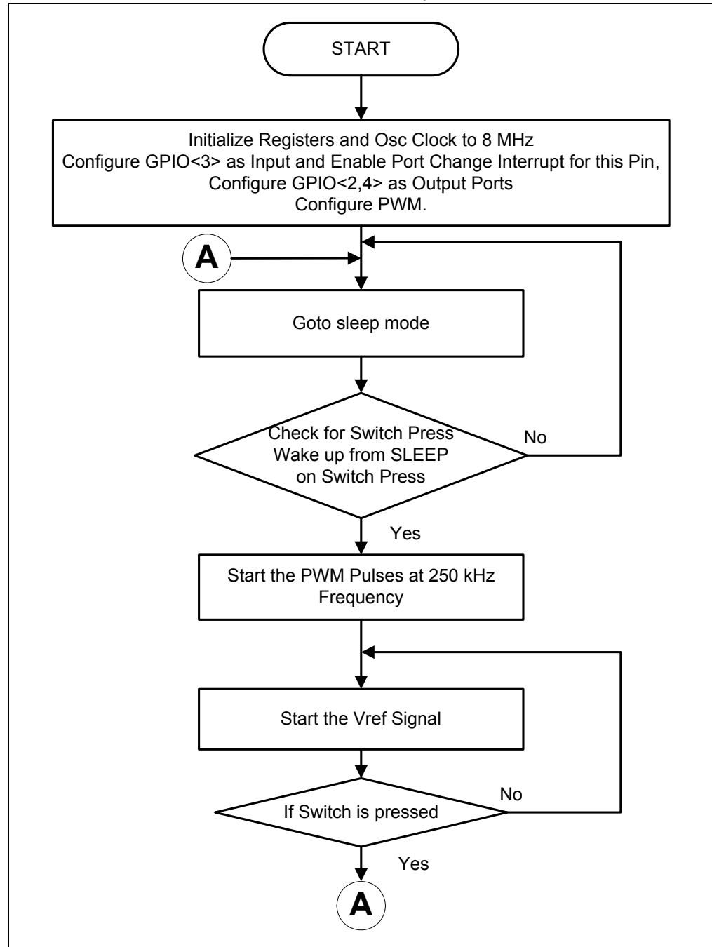
FIGURE C-1: Firmware Flowchart.
