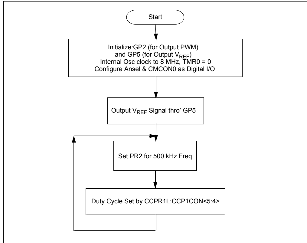
FIGURE C-1: Firmware Flowchart.
