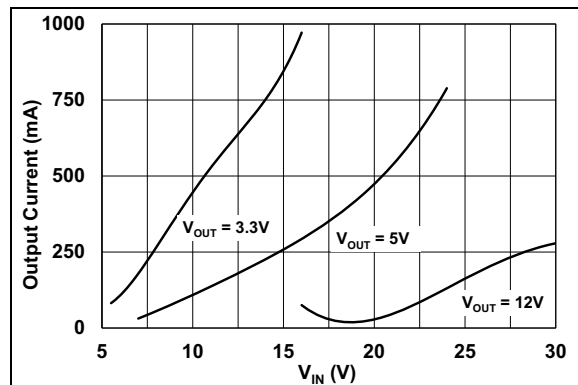
FIGURE 2-18: PFM/PWM Threshold.
