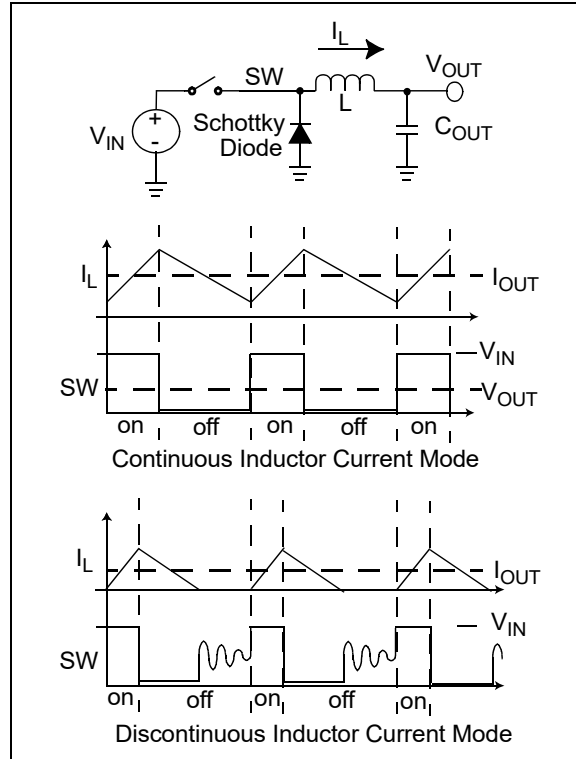
FIGURE 5-1: Step-Down Converter.
