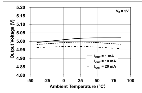
FIGURE 2-23: Output Voltage vs. Ambient Temperature.
