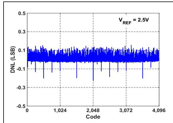
FIGURE 4-5: DNL vs. Output Code.
