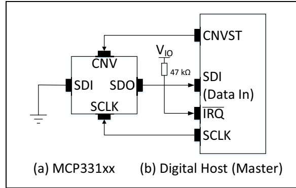
FIGURE 6-5: Connection Diagram for 3-Wire \overline{CS} Mode with BUSY Status Indicator Output Bit. IRQ Pin in the Host Device Is Used for Interrupt Event.
