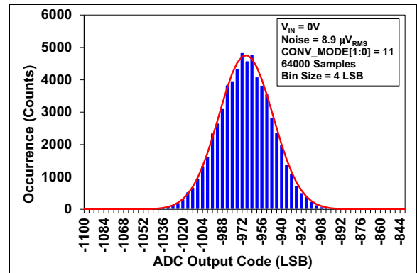
FIGURE 2-5: Output Noise Histogram (External V_{REF} ).
