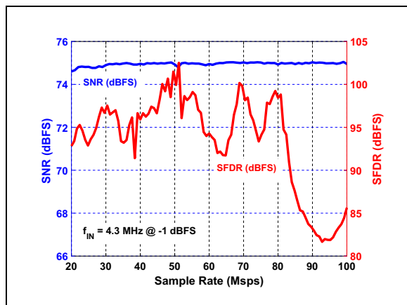
FIGURE 3-30: SNR/SFDR vs. Sample Rate (Mps): f_{IN} = 4.3 MHz.
