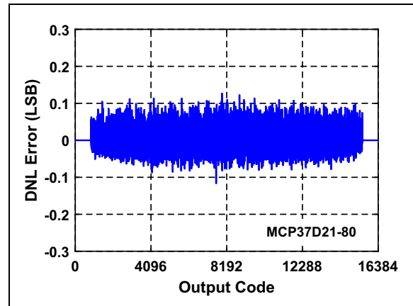
FIGURE 3-44: DNL Error Vs. Output Code: f_S = 80 \text{ Msps} , f_{IN} = 4.3 \text{ MHz} , A_{IN} = -1\text{dBFS} , MCP37D21-80.
