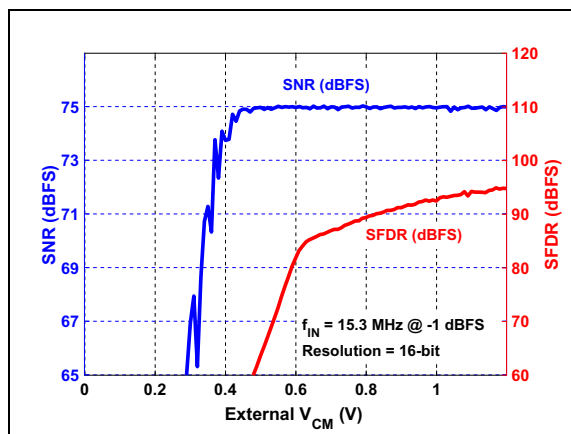
FIGURE 3-34: SNR/SFDR vs. V_{CM} Voltage (Externally Applied): f_S = 80 Mps, f_{IN} = 15.3 MHz.
