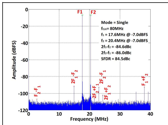
FIGURE 3-29: Two-Tone FFT. MCP37D31-80.
