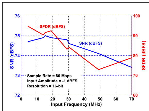
FIGURE 3-31: SNR/SFDR vs. Input Frequency: f_S = 80 Mps.
