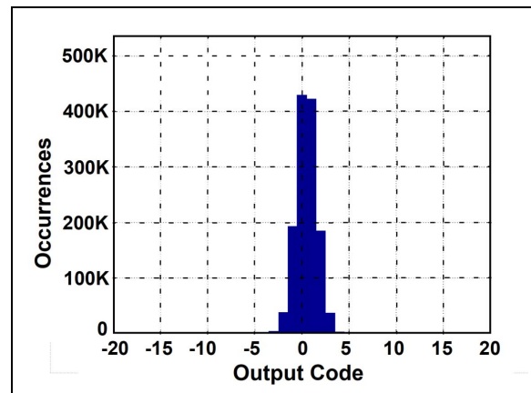
FIGURE 3-45: Shorted Input Histogram: f_S = 80 \text{ Msps} , MCP37D21-80.
