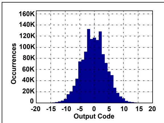
FIGURE 3-42: Shorted Input Histogram: f_S = 80 \text{ Msps} , MCP37D31-80.
