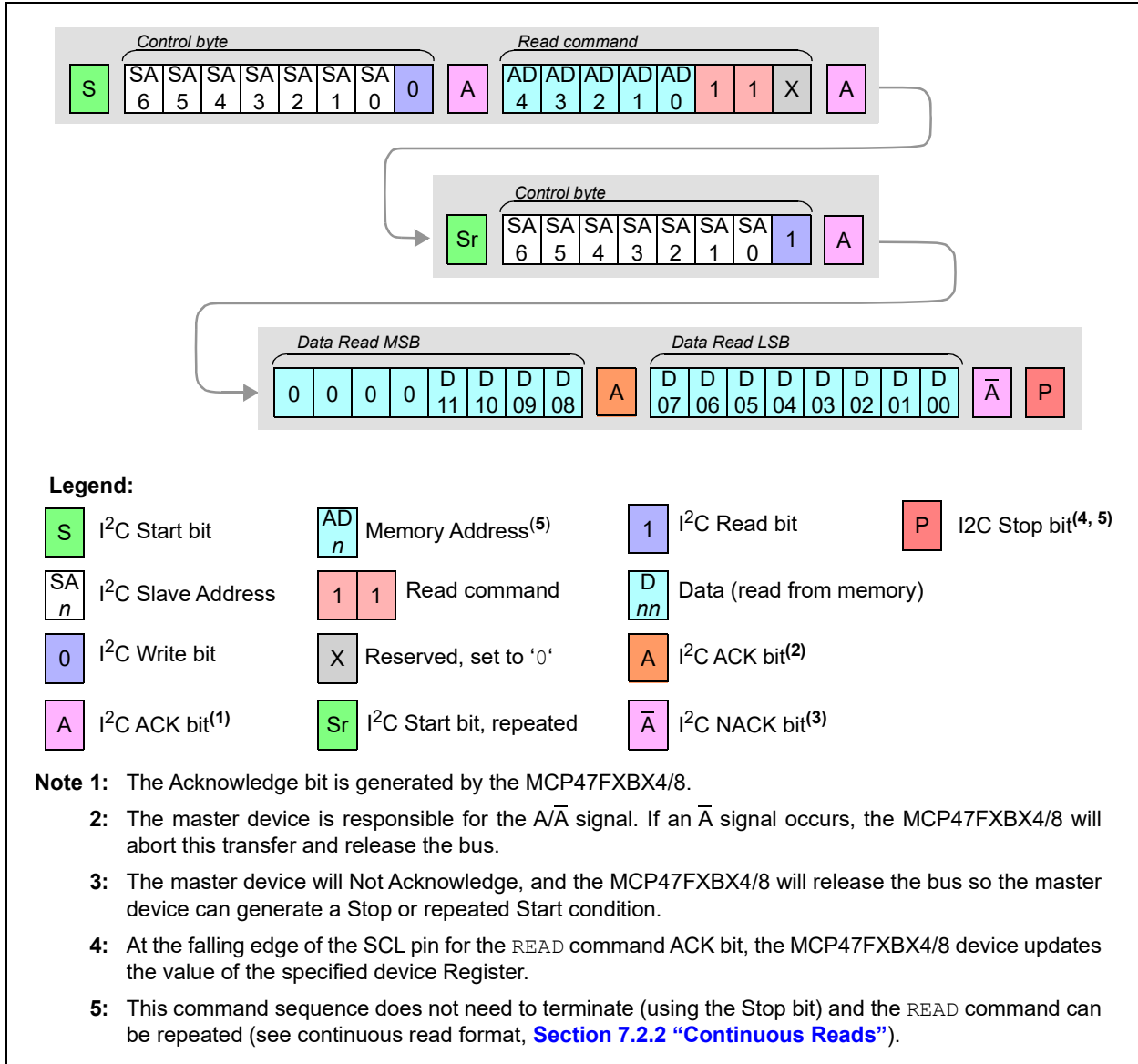
FIGURE 7-4: READ Command – Single Memory Address.
