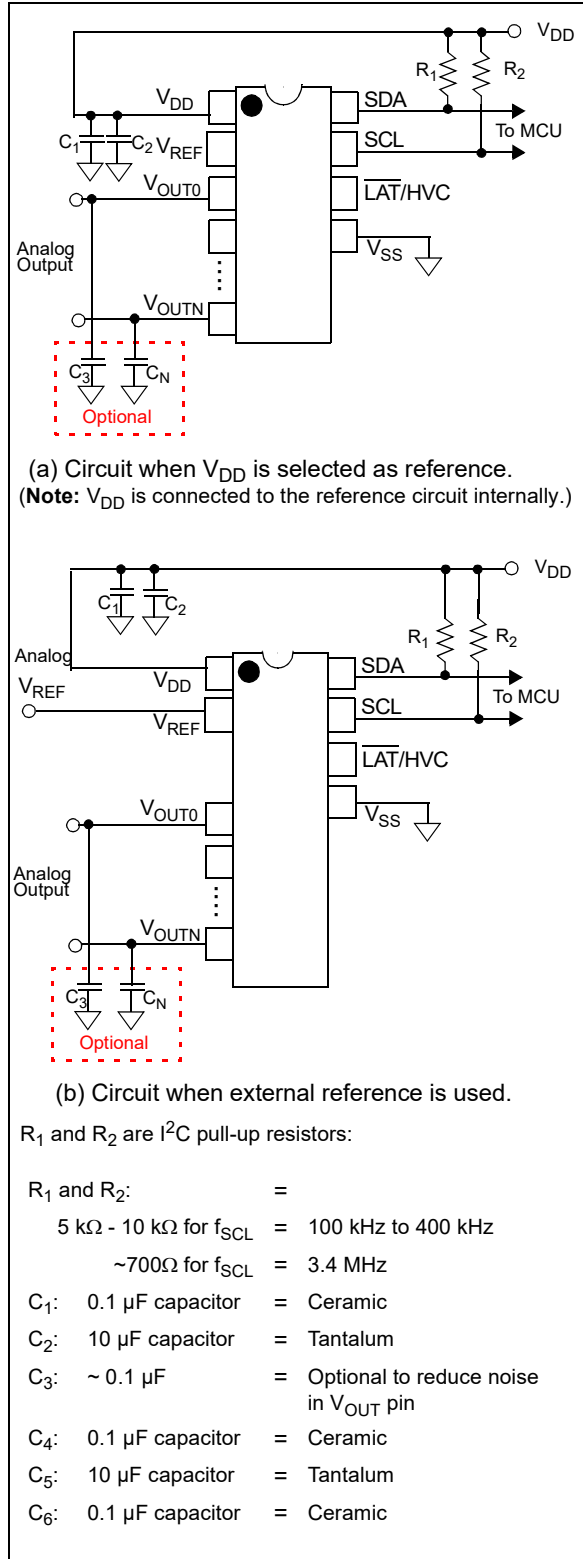
FIGURE 8-3: Circuit Example.
