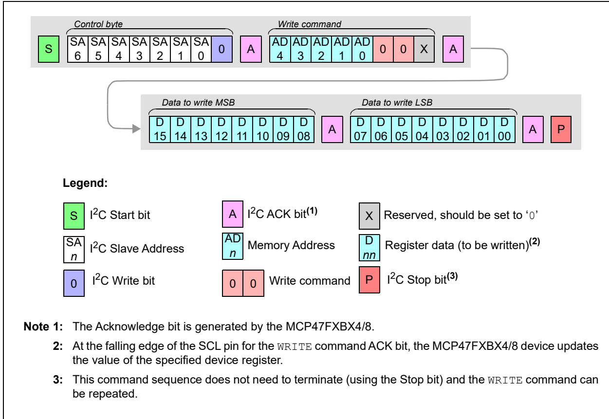
FIGURE 7-1: Write Random Address Command (Volatile and Nonvolatile Memory).
