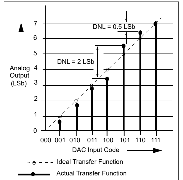
FIGURE C-5: DNL ACCURACY.
