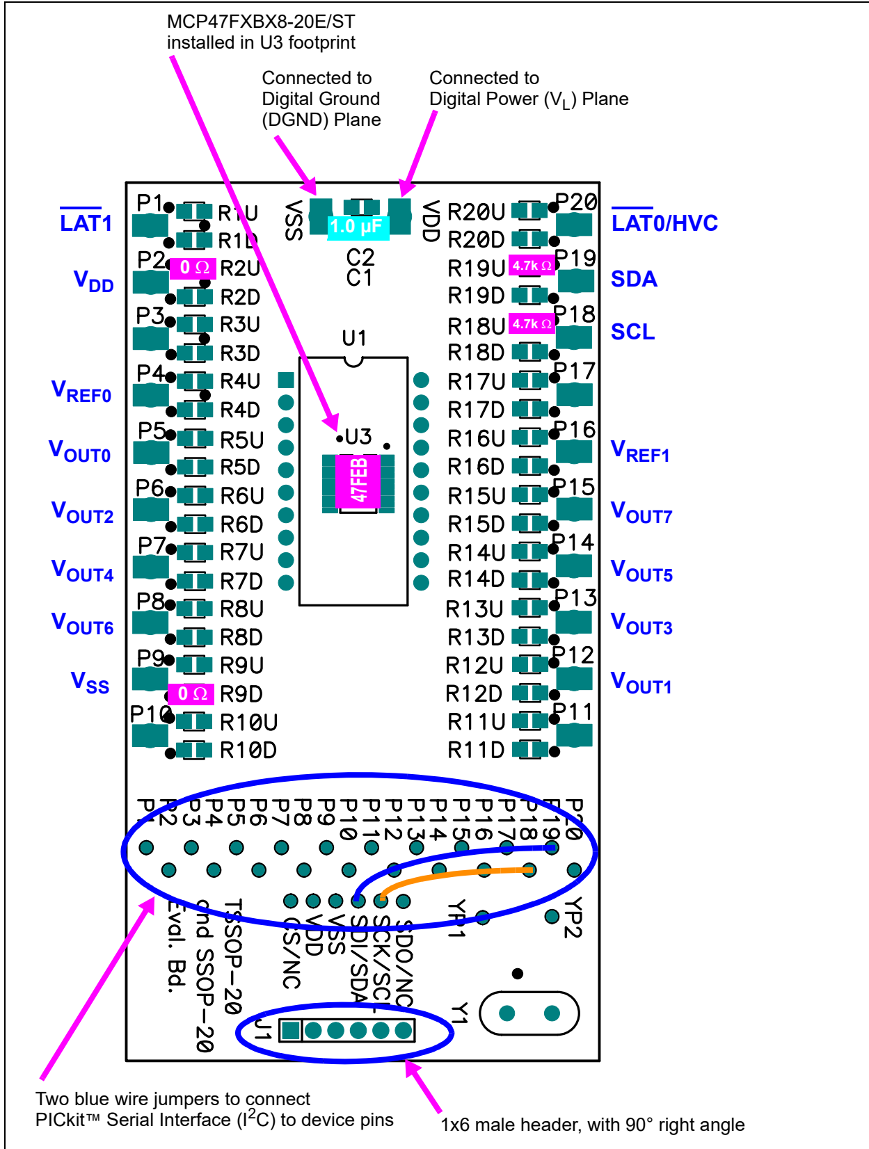
FIGURE 9-1: MCP47FBX4/8 Evaluation Board Circuit Using TSSOP20EV.
