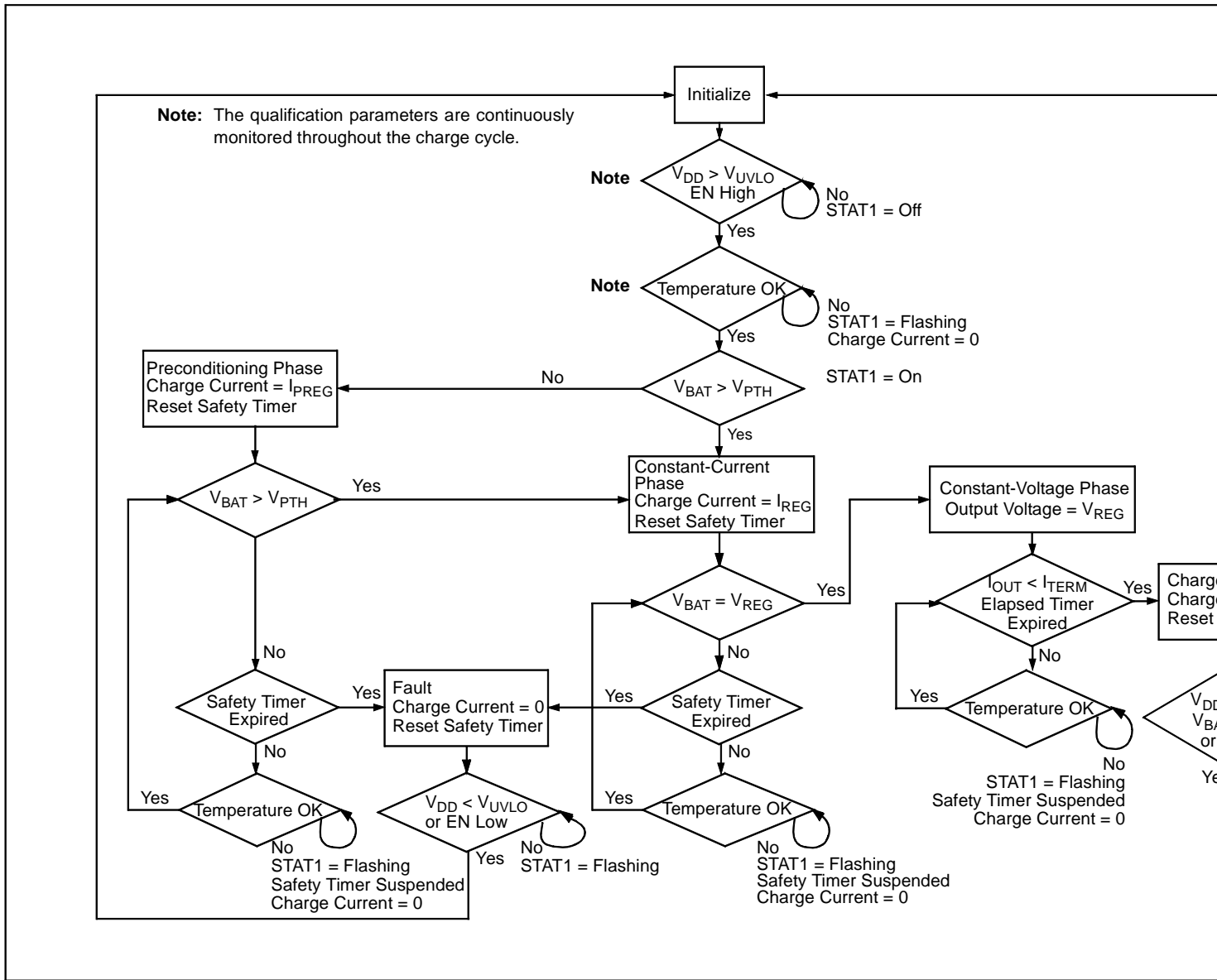
FIGURE 4-1: Operational Flow Algorithm - MCP73841 and MCP73842.
