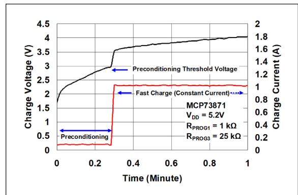
FIGURE 2-29: Typical Charge Profile in Preconditioning (1000 mAh Battery).
