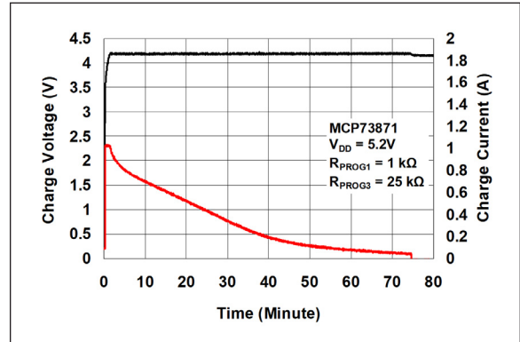
FIGURE 2-28: Complete Charge Cycle (1000 mAh Li-Ion Battery).
