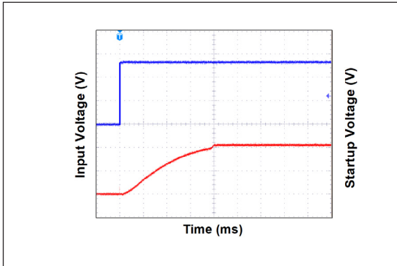
FIGURE 2-25: Start-up Delay.
