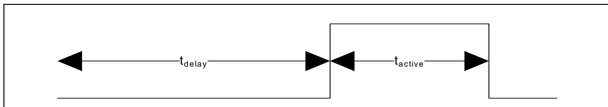
FIGURE 57-9: KBRST TIMING
