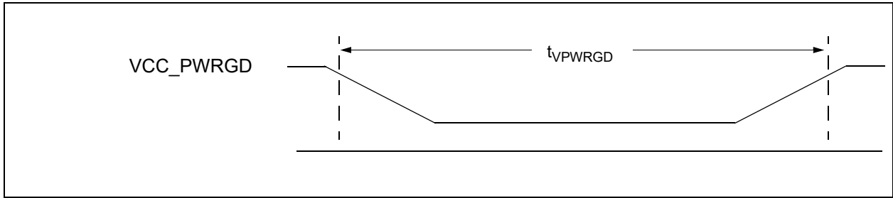
FIGURE 57-4: VCC_PWRGD TIMING
