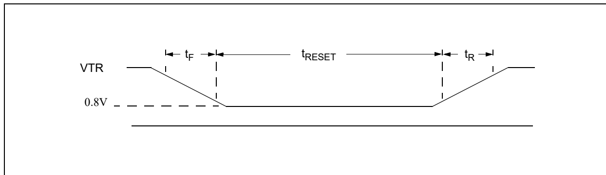
FIGURE 57-5: NRESET_IN TIMING
