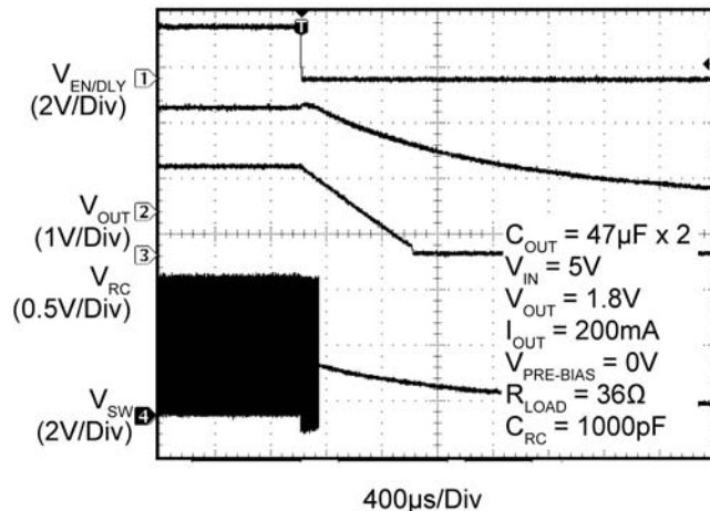
Figure 6. EN Turn-Off - 200mA Load
