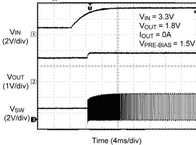
V IN Start-up with Pre-Biased Output
