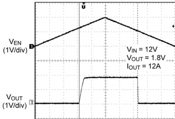
Enable Thresholds
