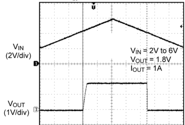
V_{IN} UVLO Thresholds
