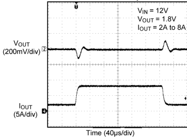
Transient Response
