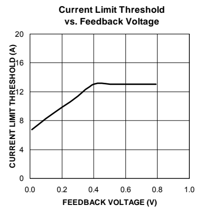
Figure 5. MIC26903 Current Limit Foldback Characteristic
