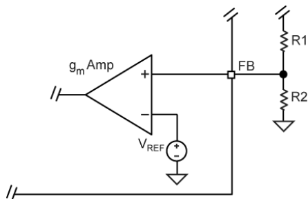
Figure 7. Voltage-Divider Configuration
