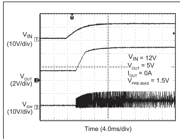
FIGURE 4-6: MIC28304-1 V_{IN} Start-up with Pre-Biased Output.
