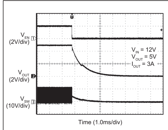
FIGURE 4-4: Enable Turn-Off Delay and Fall Time.
