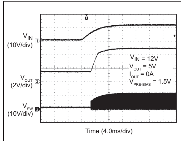
FIGURE 4-5: MIC28304-2 V_{IN} Start-up with Pre-Biased Output.
