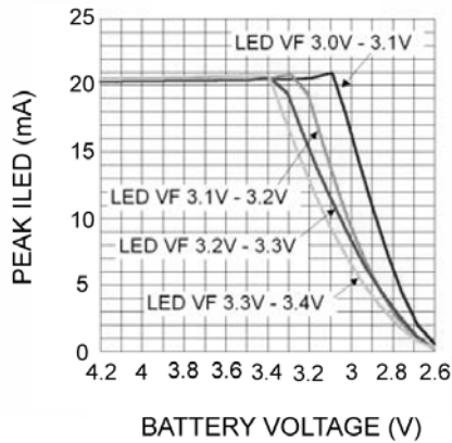
20mA Peak ILED vs. Battery Voltage
