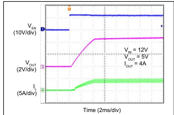
FIGURE 2-28: Enable Turn-On.
