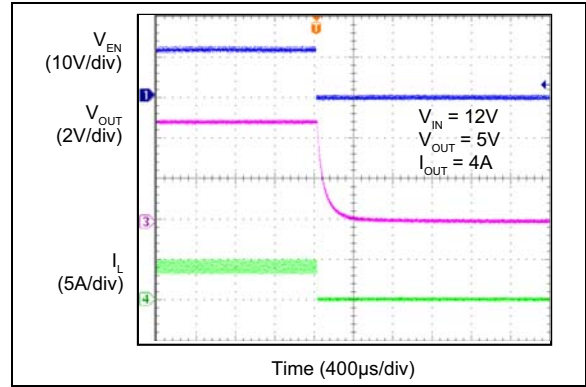
FIGURE 2-29: Enable Turn-Off.
