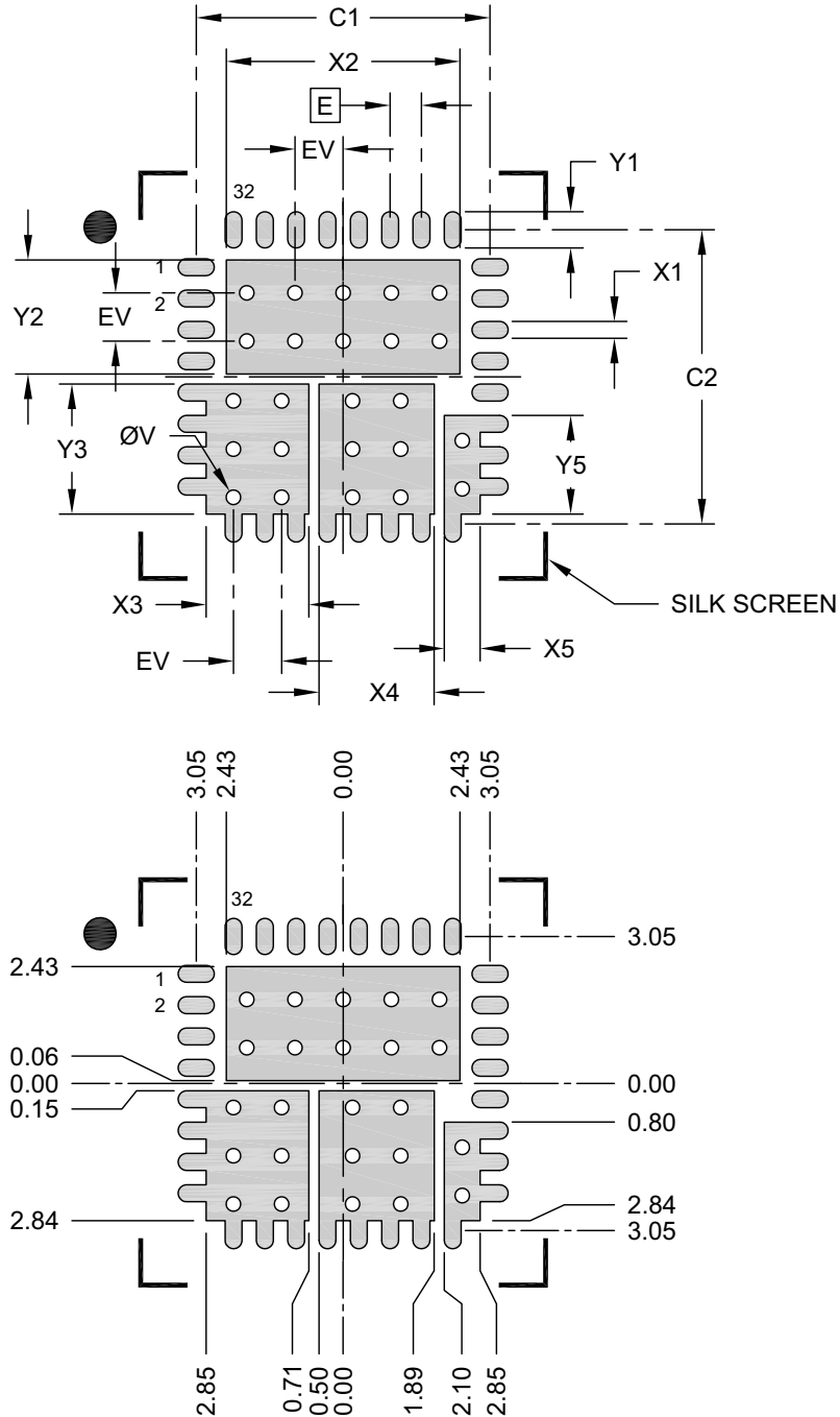
Microchip Technology Drawing C04-3196 Rev C Sheet 1 of 2
