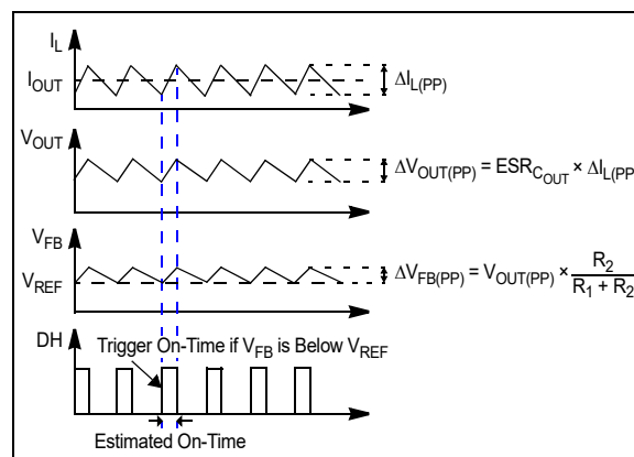
FIGURE 4-1: MIC28516 Control Loop Timing.
