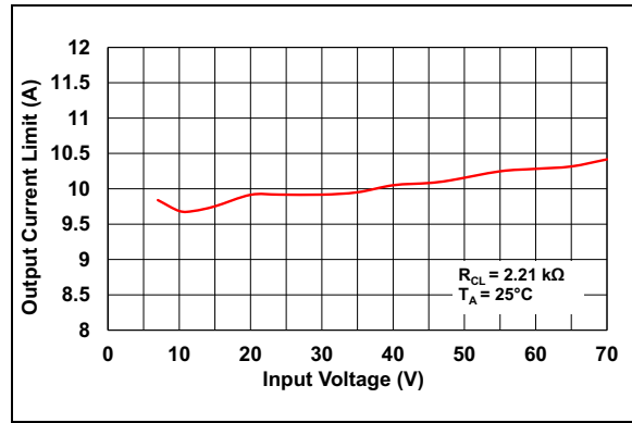
FIGURE 2-34: Output Current Limit vs. Input Voltage.
