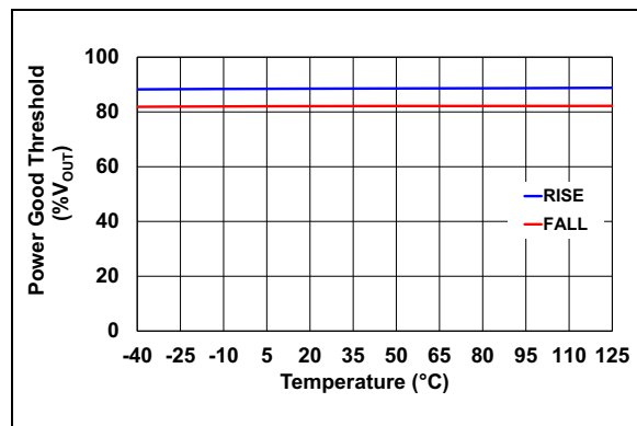
FIGURE 2-36: Power Good Threshold vs. Temperature.
