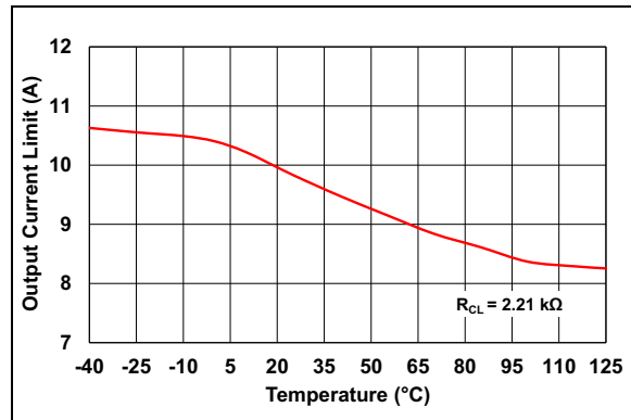
FIGURE 2-35: Output Current Limit vs. Temperature.
