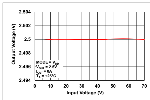
FIGURE 2-11: Output Voltage vs. Input Voltage ( V_{OUT} = 2.5V ).
