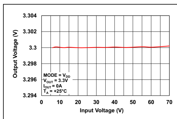
FIGURE 2-12: Output Voltage vs. Input Voltage ( V_{OUT} = 3.3V ).
