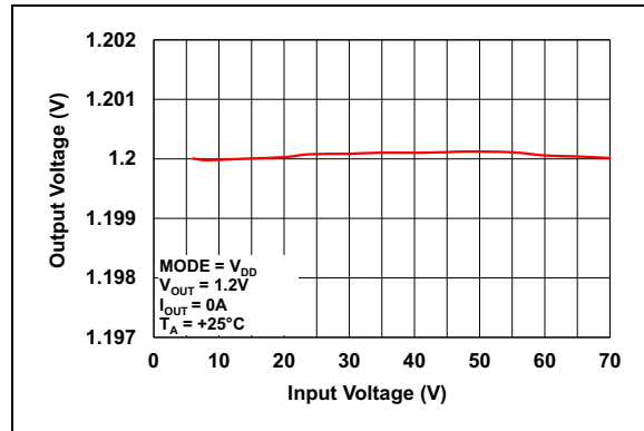
FIGURE 2-10: Output Voltage vs. Input Voltage ( V_{OUT} = 1.2V ).
