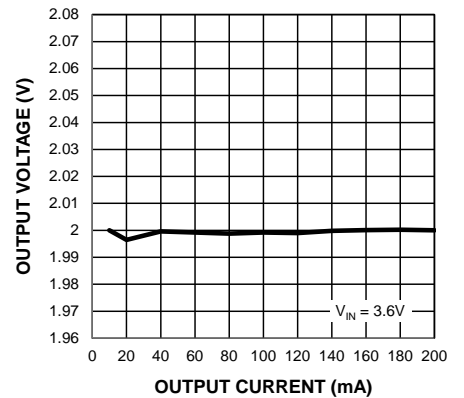
Output Voltage vs. Output Current (DCM)
