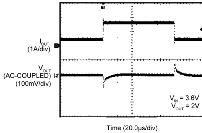
Load Transient (250mA – 1.5A)
