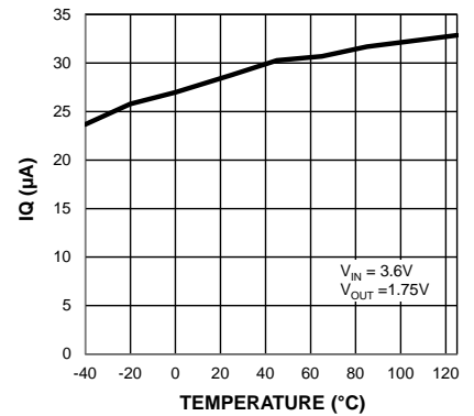
Quiscent Current vs. Temperature
