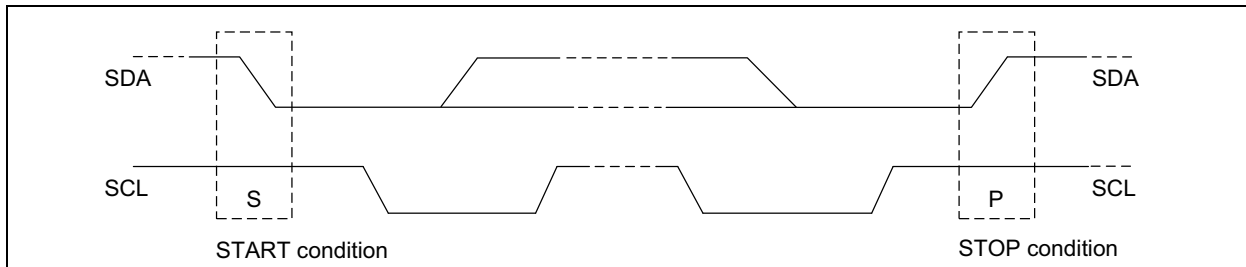
FIGURE 6-2: Start and Stop Conditions.
